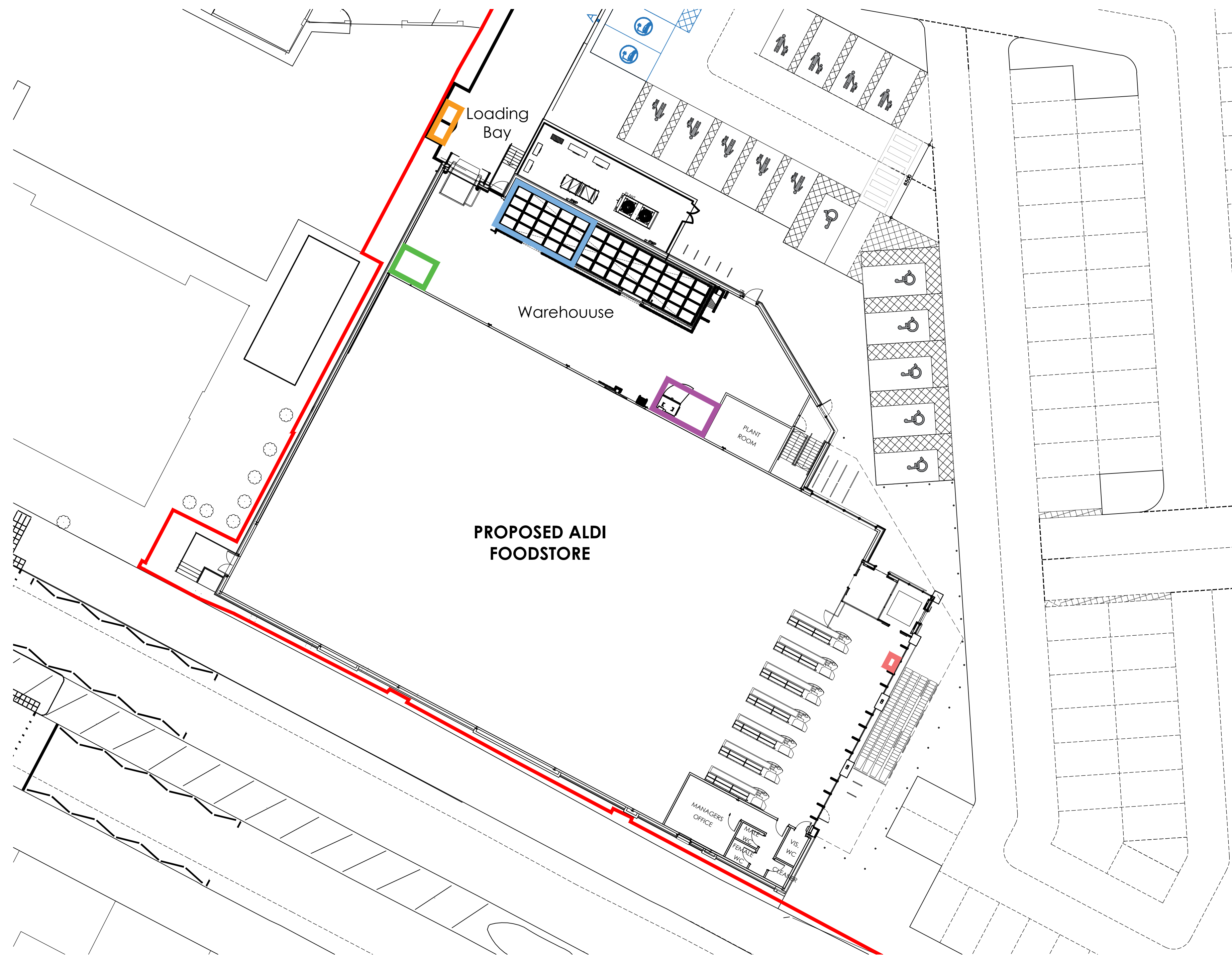
PROPOSED REFUSE PLAN - 1:200
