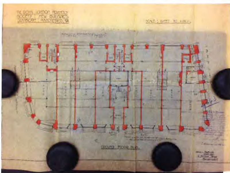
Fig 12: Archive Ground Floor Plan
