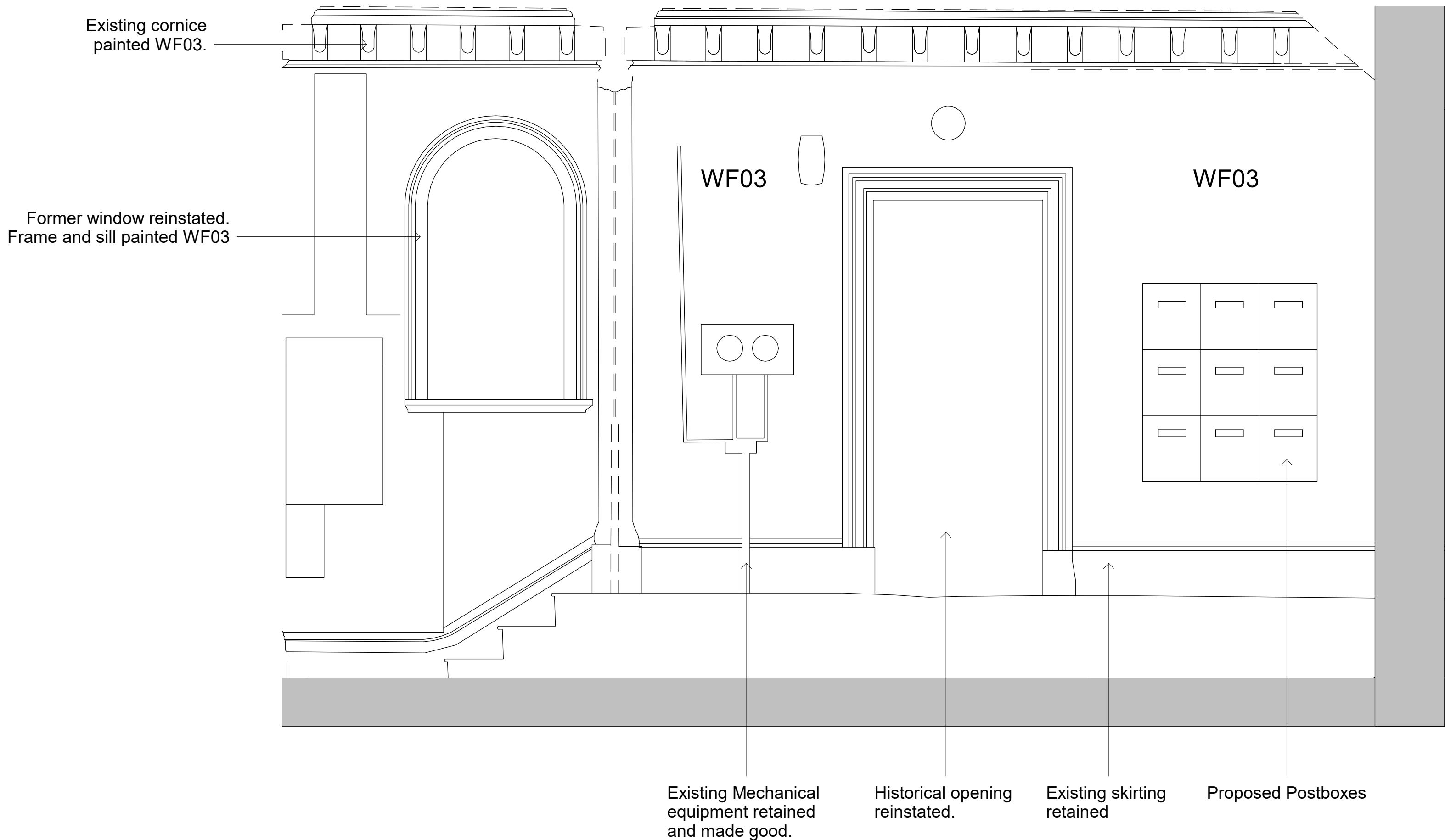
GFL - Elevation 8 1 : 20
