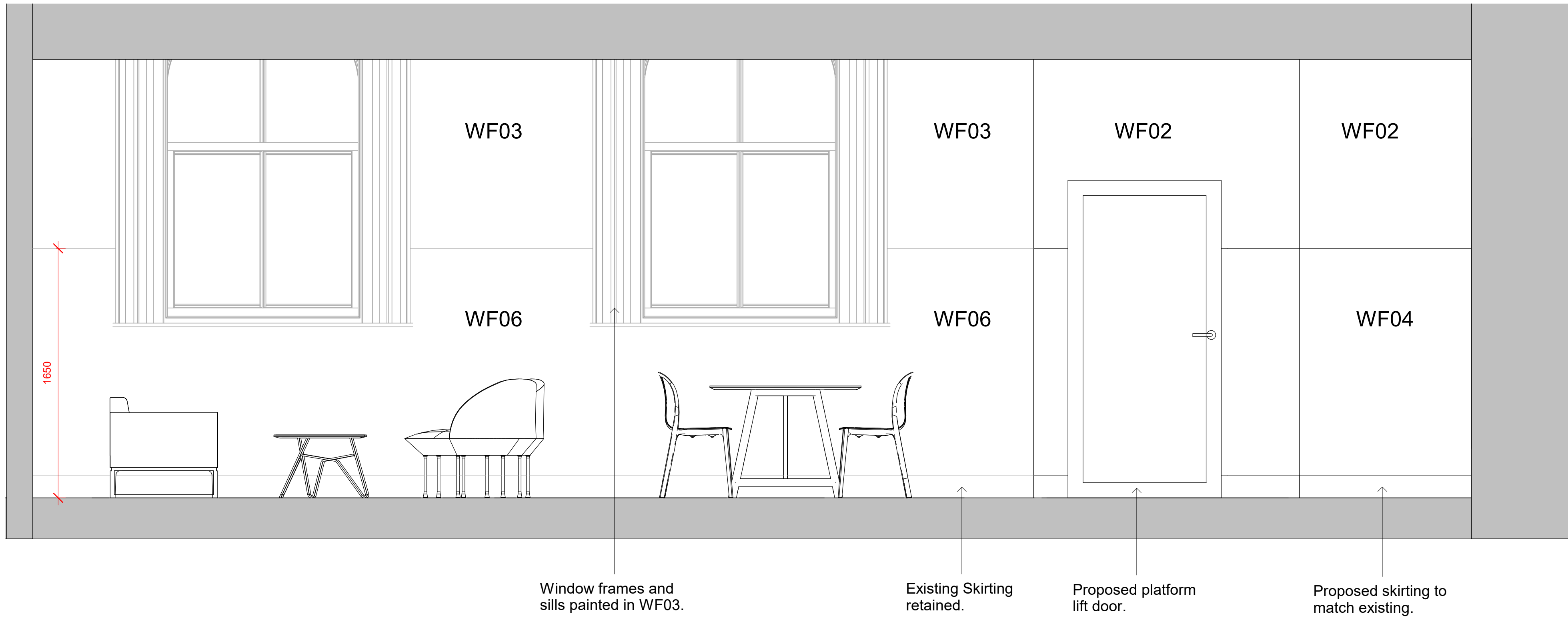
GFL - Elevation 10 1 : 20
