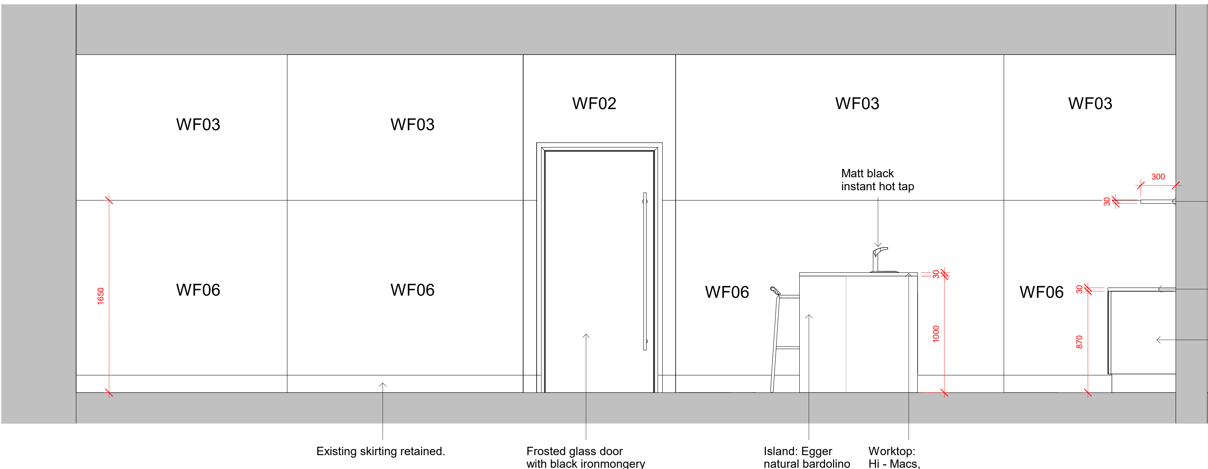
GFL - Elevation 6 1 : 20
