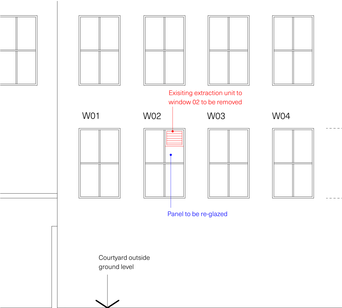
EXTERNAL ELEVATION TO WINDOWS FROM EXISTING REAR COURTYARD
