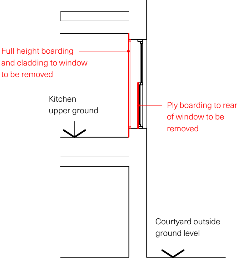
EXISTING SECTION WINDOWS 03 & 04
