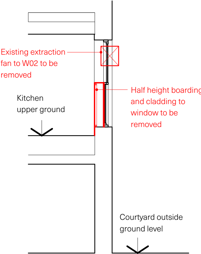
EXISTING SECTION WINDOWS 01 & 02
