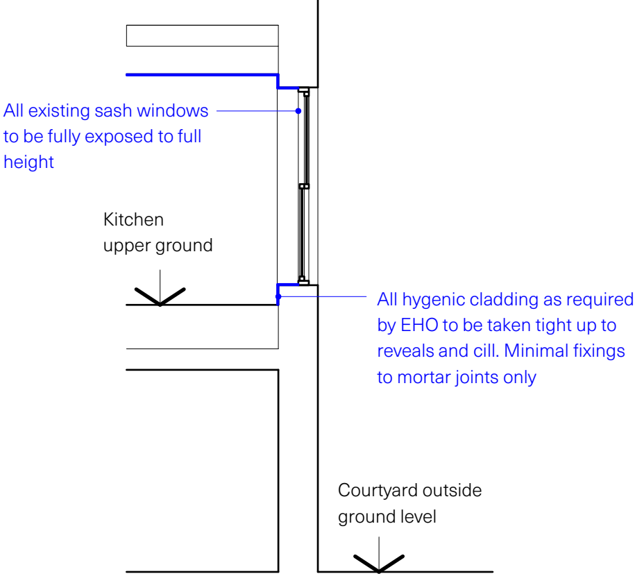
PROPOSED SECTION TO ALL WINDOWS
