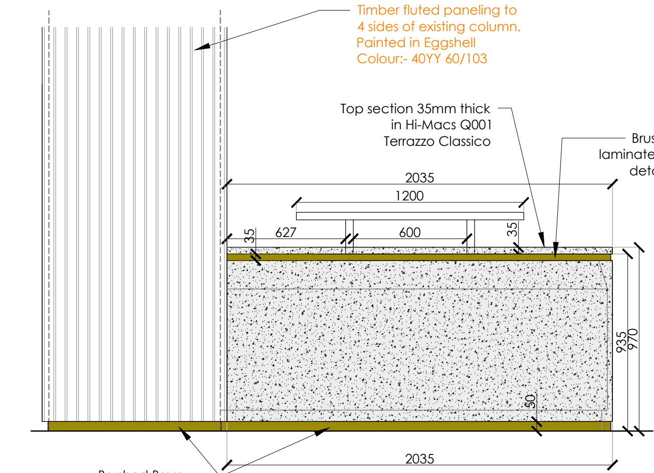
PROPOSED ELEVATION A SCALE 1:20
