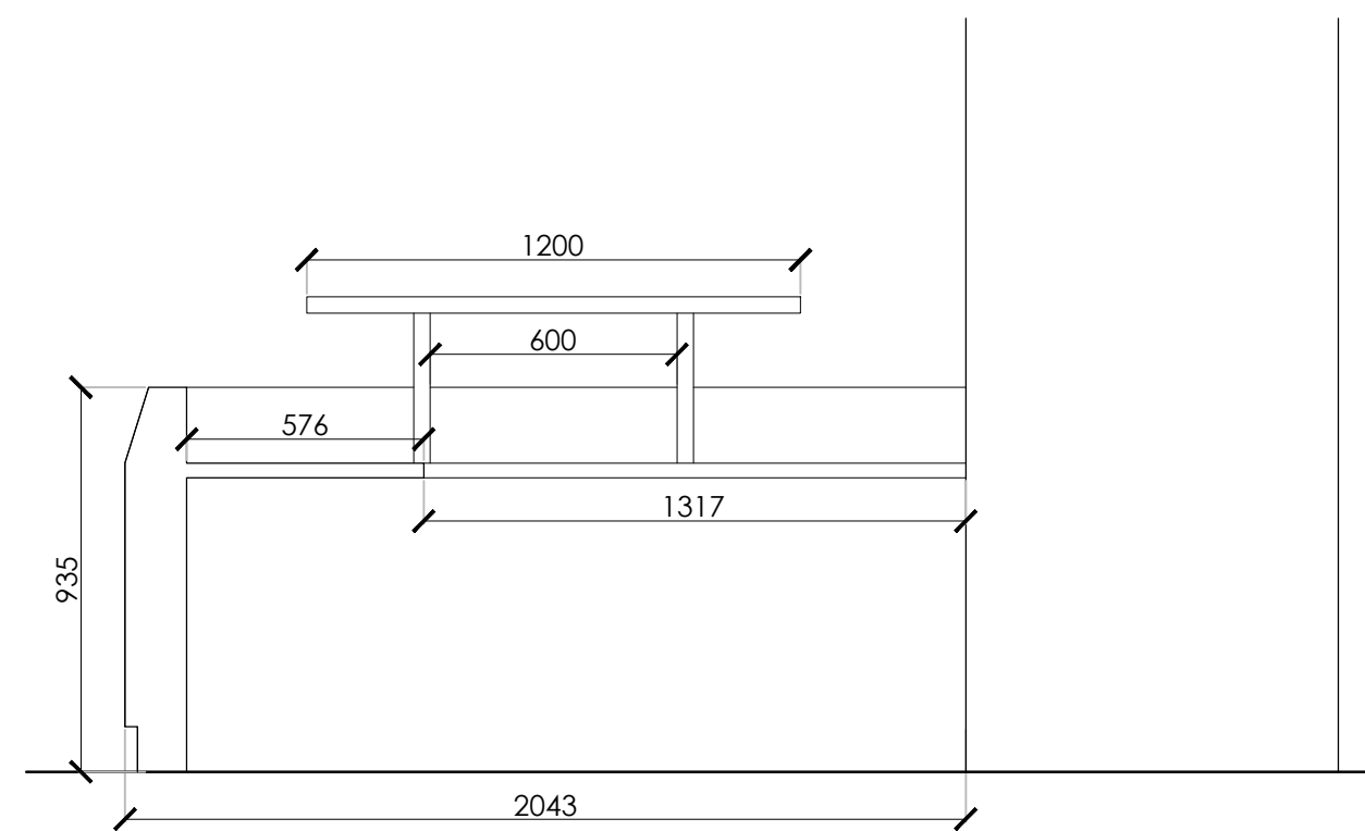
EXISTING ELEVATION C SCALE 1:20
