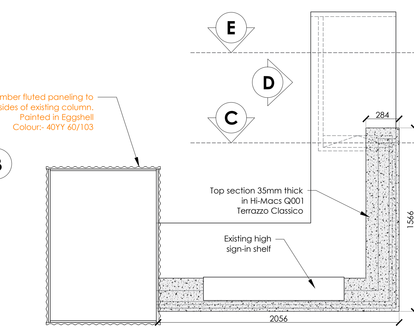
RECEPTION DESK PROPOSED PLAN SCALE 1:20
