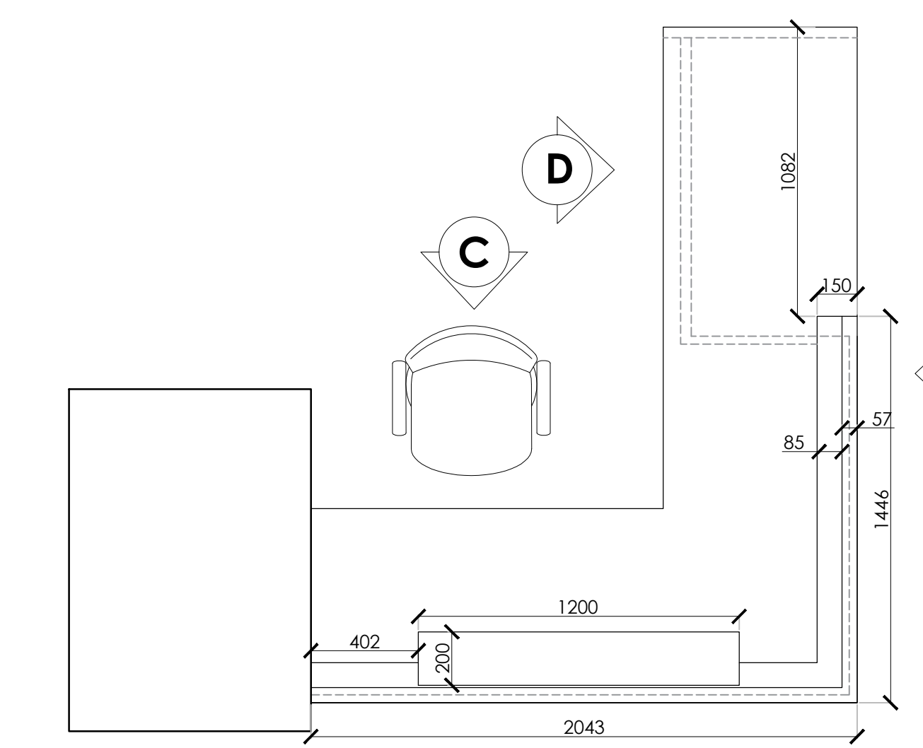
RECEPTION DESK EXISTING PLAN SCALE 1:20
