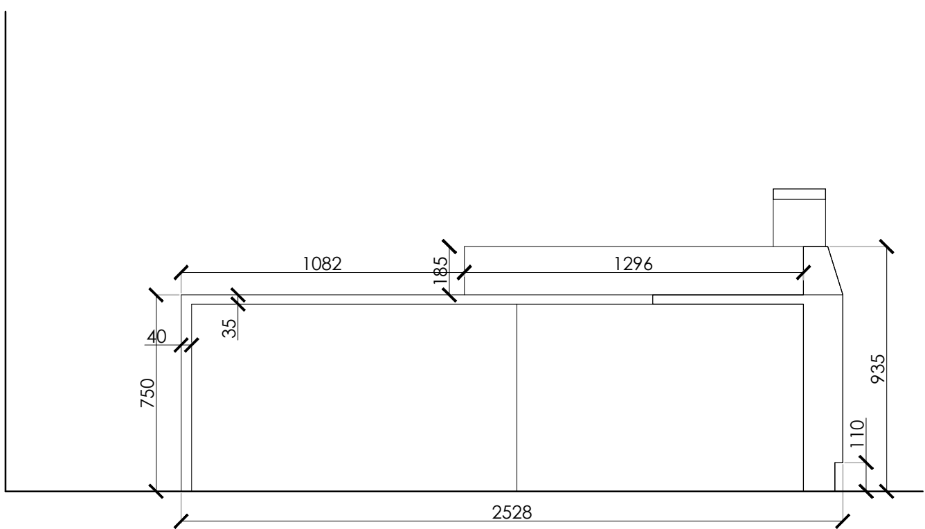
EXISTING ELEVATION D SCALE 1:20
