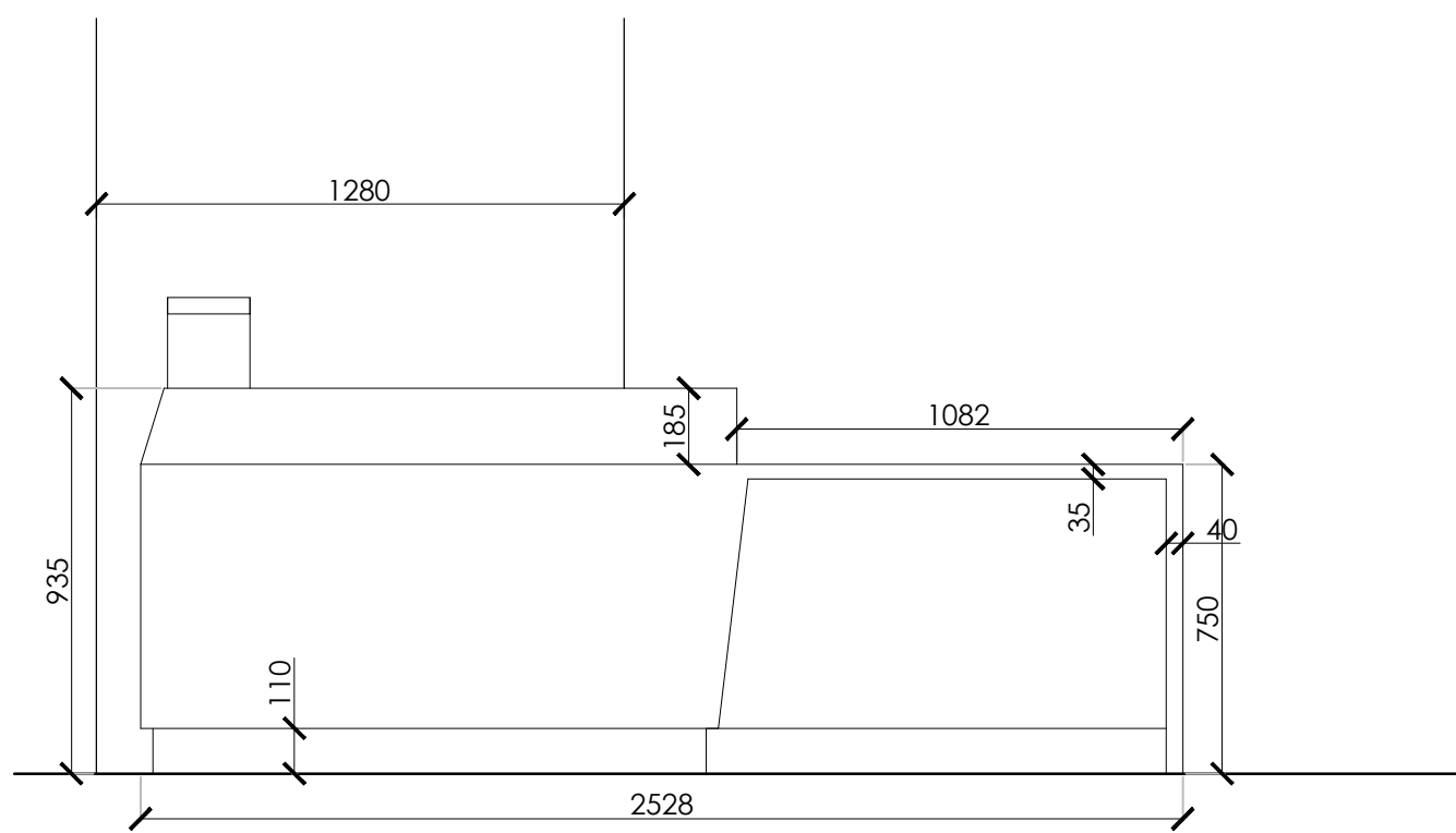
EXISTING ELEVATION B SCALE 1:20
