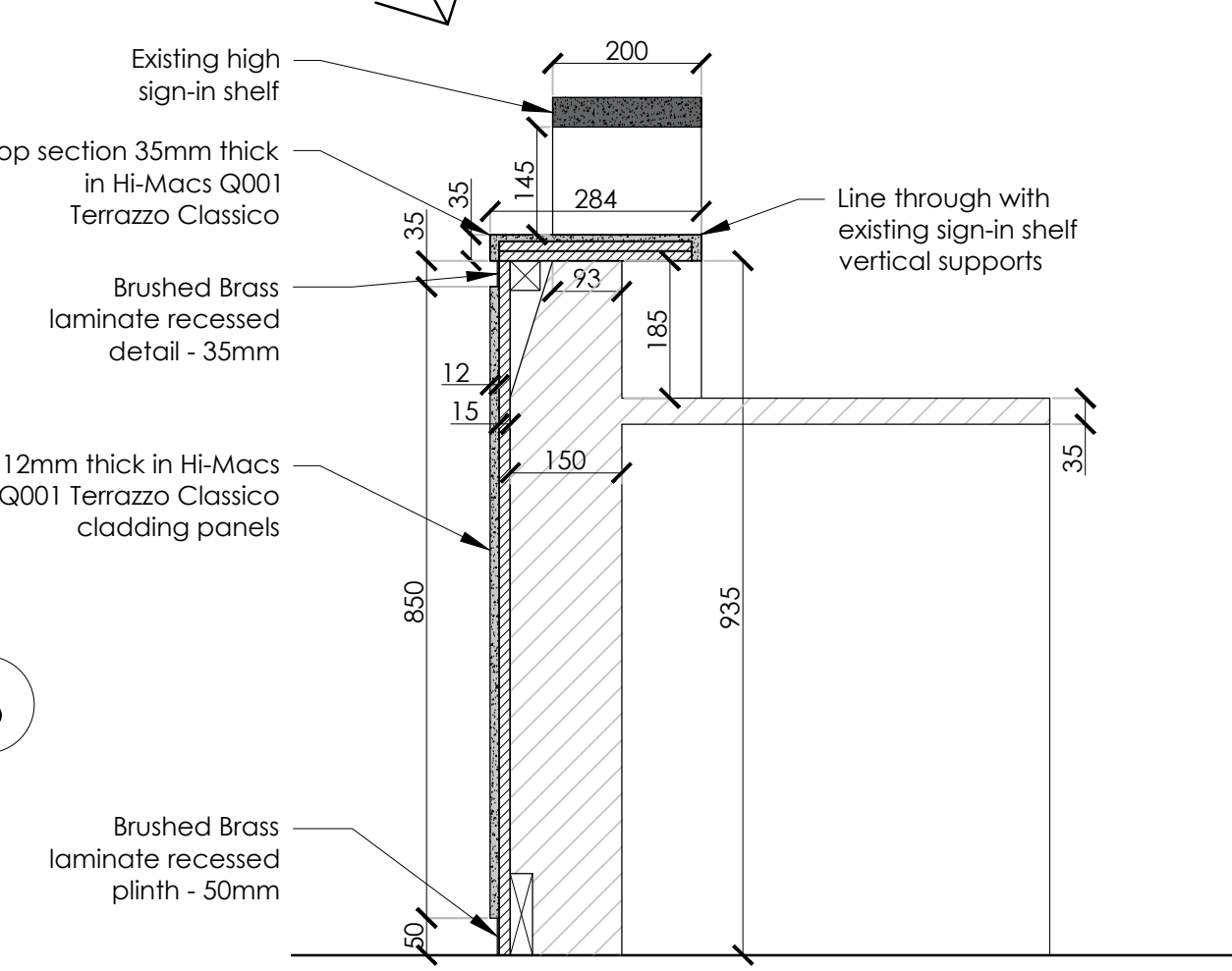
SECTION DETAIL THROUGH RE-CLAD RECEPTION DESK SCALE 1:10
