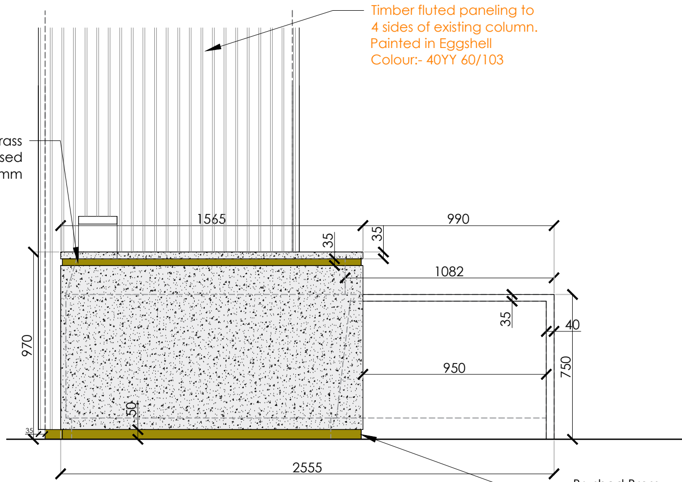
PROPOSED ELEVATION B SCALE 1:20
