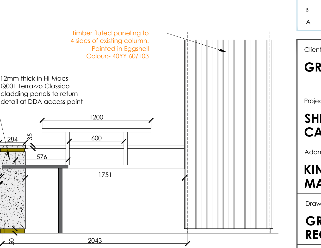
PROPOSED ELEVATION E SCALE 1:20
