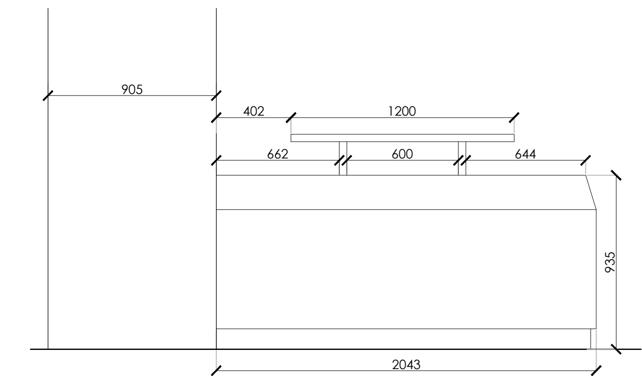
EXISTING ELEVATION A SCALE 1:20
