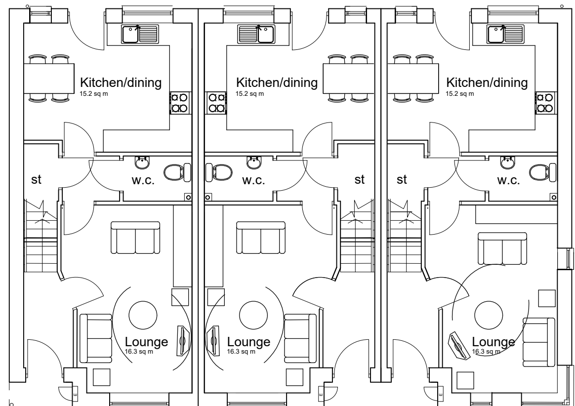
Ground floor
