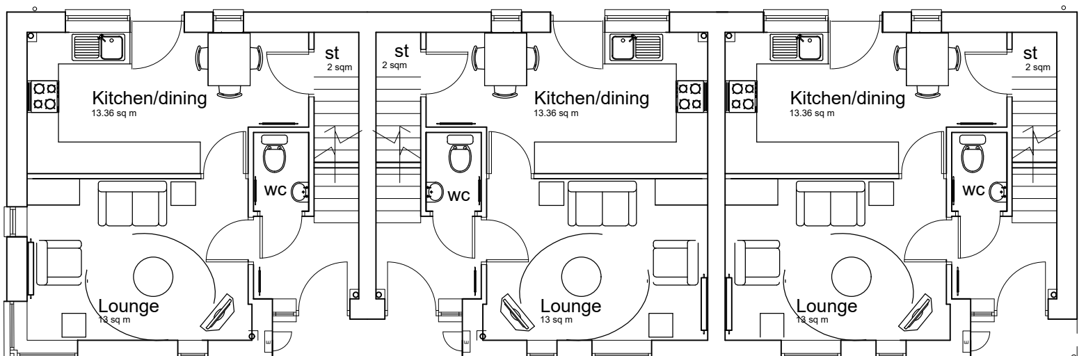
Ground floor
