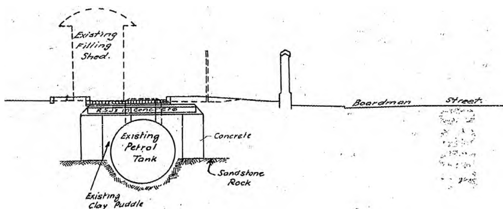
Fig 3.0: Extract from LMSR Plan relating to Road Motor Petrol Depot improvement works
