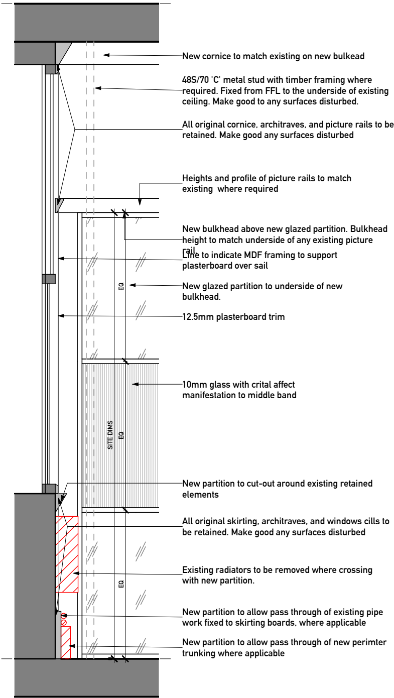
2 Typical Abutment Detail Section XX-700 1 : 20
