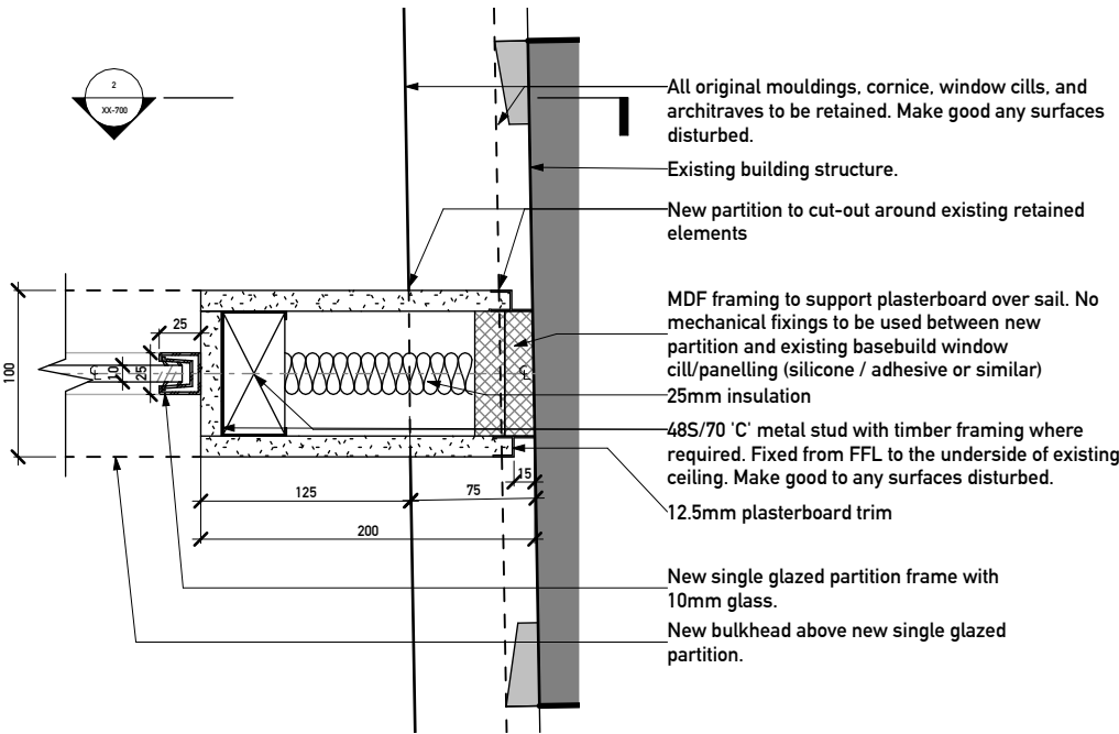
1 Typical Abutment Detail - Plan 02-110 1 : 5
