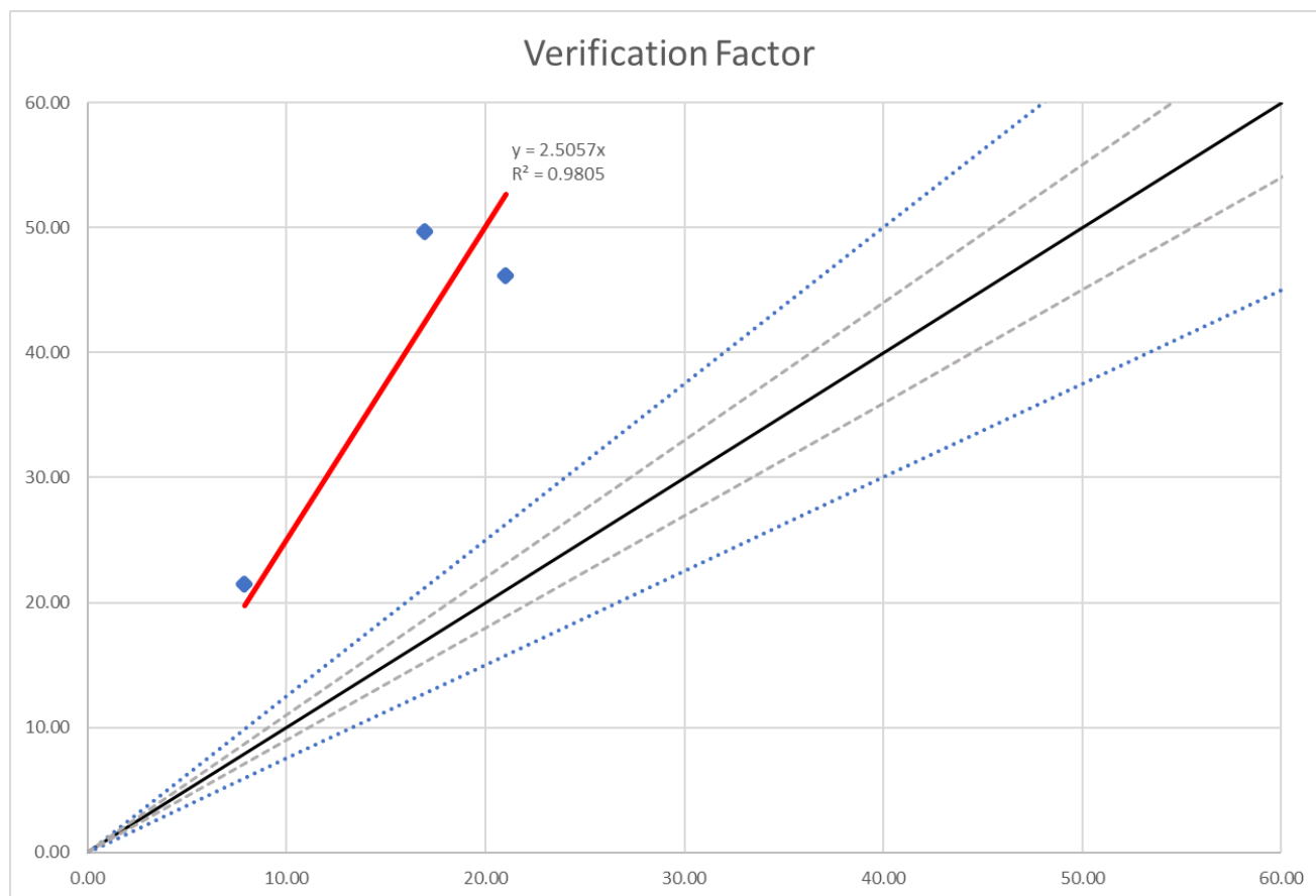
Figure 8: Initial Comparison of Measured Road NO x to Unadjusted Modelled Road NO x Concentrations
