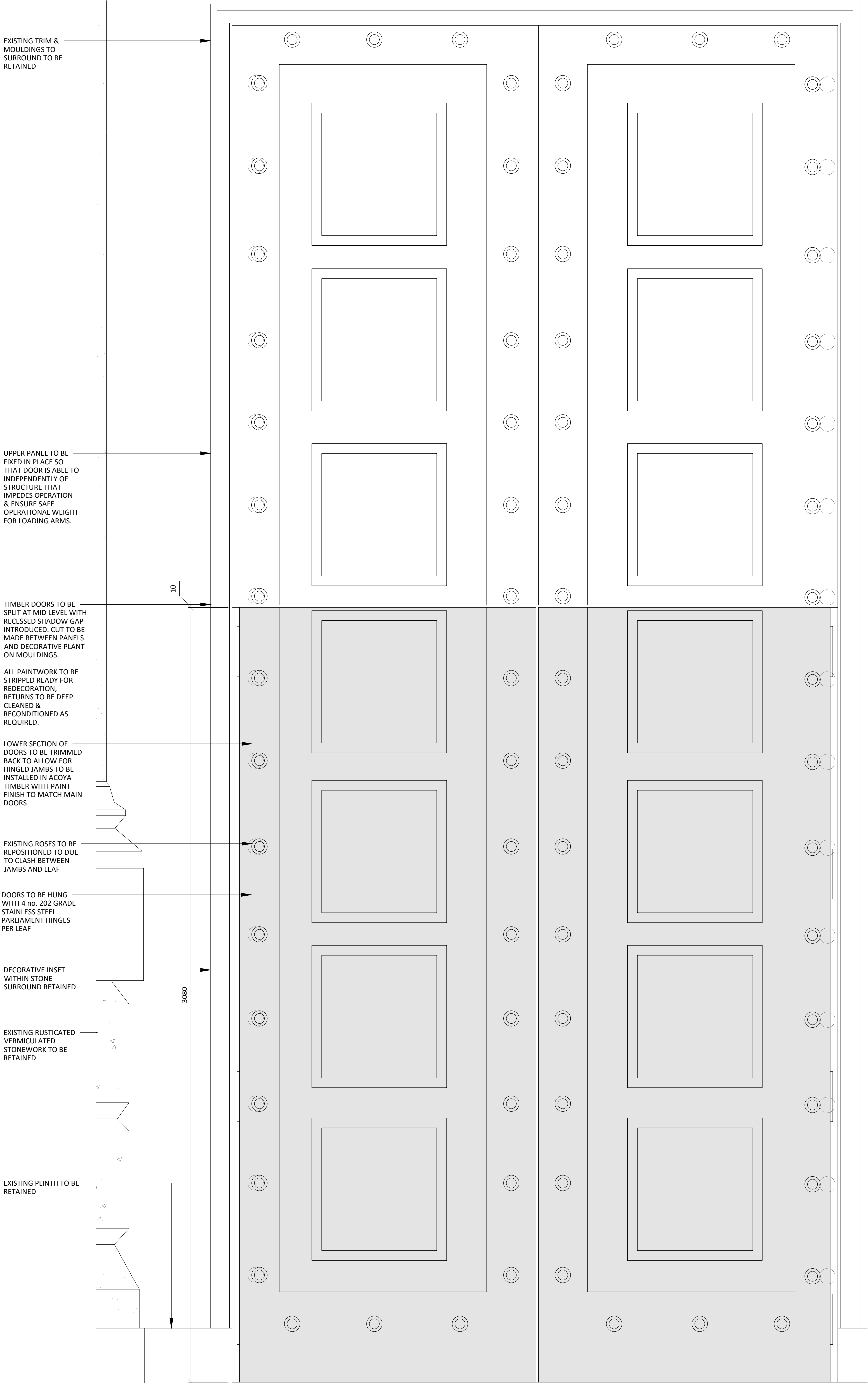
01 EXTERNAL DOOR ELEVATION 536 SCALE - 1:10 @ A1 AS PROPOSED
