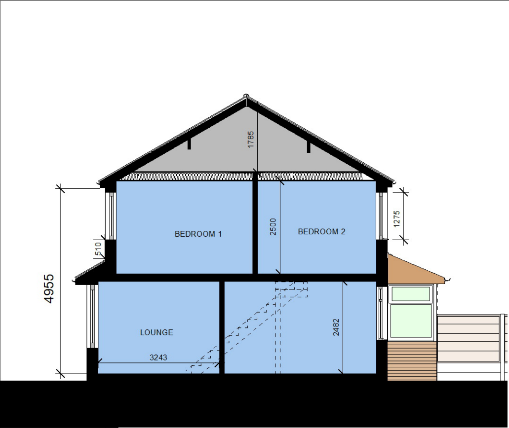
SECTION A-A AND SIDE ELEVATION AS EXISTING
