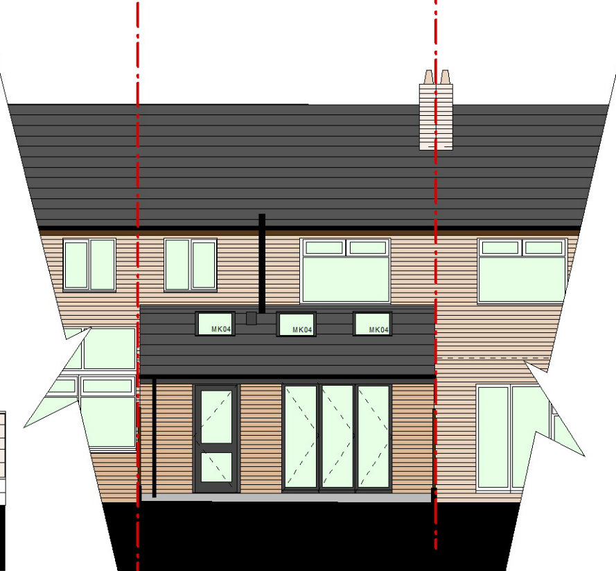
BACK ELEVATION AS PROPOSED (SOUTH)
