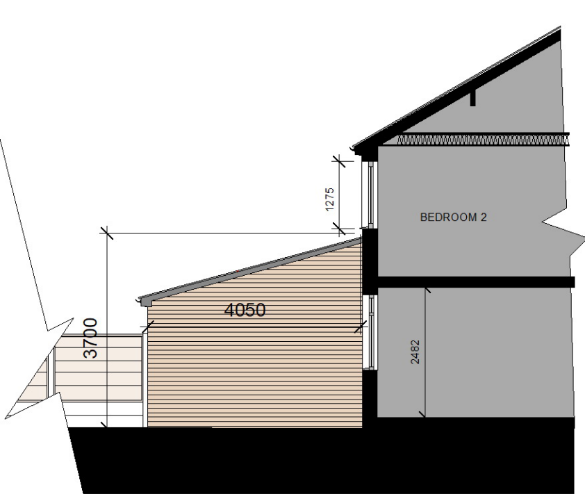
SIDE ELEVATION TO NO.12 AS PROPOSED (EAST)
