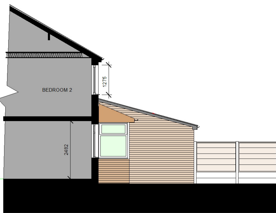
SIDE ELEVATION TO NO.8 AS PROPOSED (WEST)
