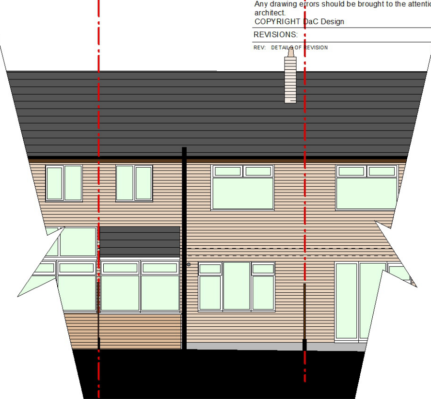
BACK ELEVATION AS EXISTING (SOUTH)
