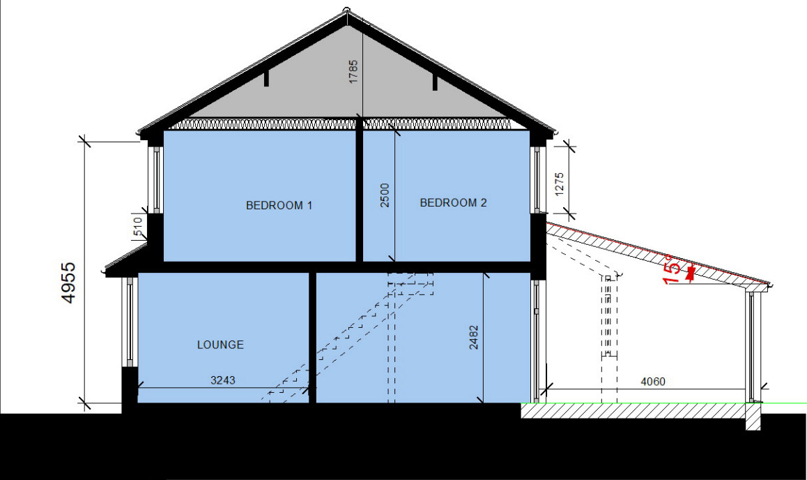
SECTION A-A AS PROPOSED
