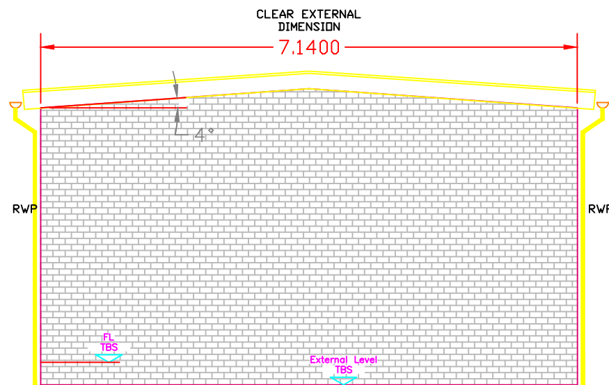
Proposed Substation Side Elevation D
