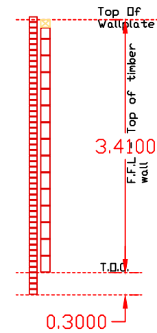
Proposed Substation Rear Elevation B
