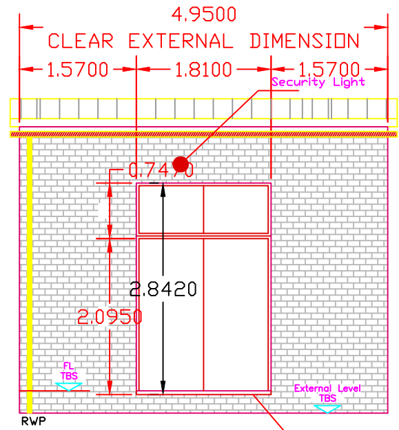
Proposed Substation Front Elevation A
