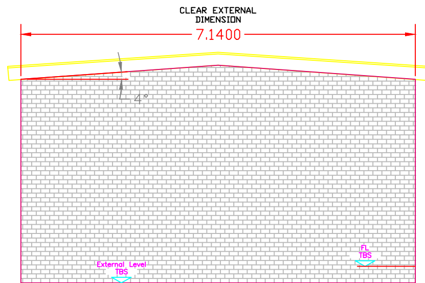
Proposed Substation Side Elevation C
