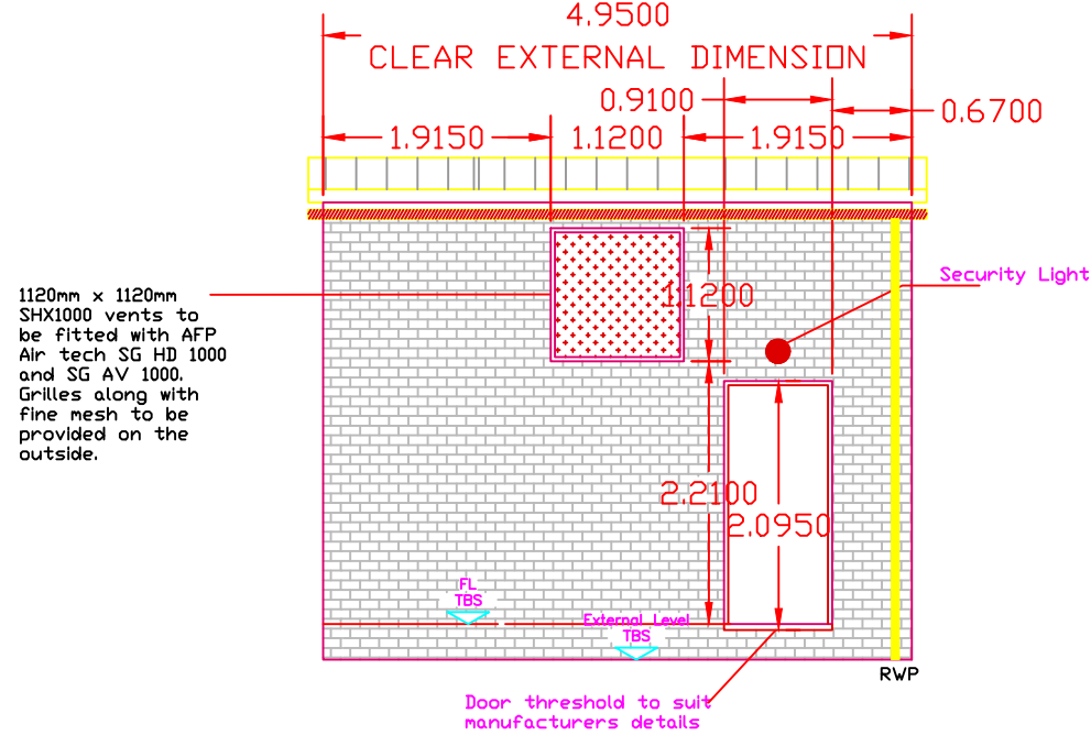
Proposed Substation Rear Elevation B
