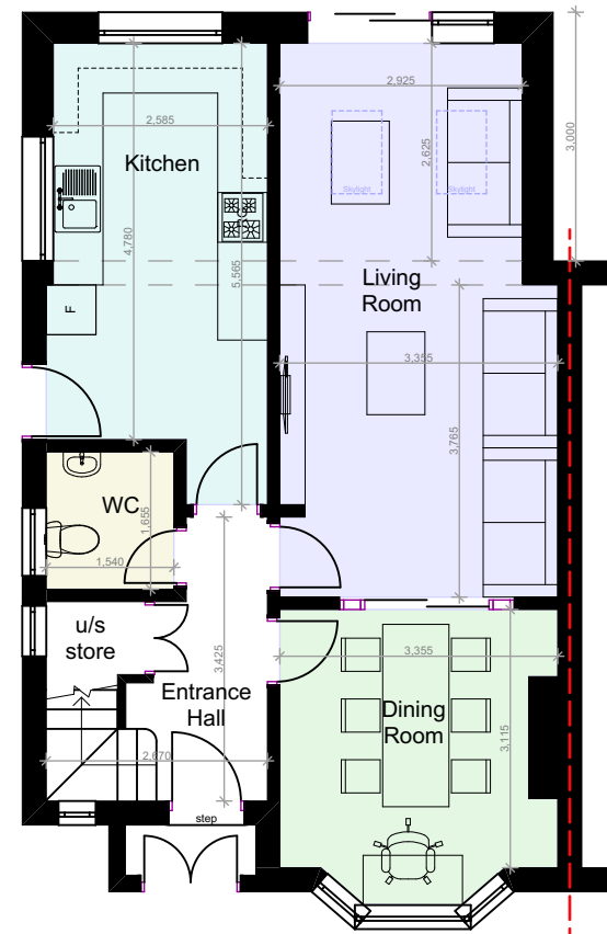
PROPOSED GA GROUND FLOOR PLAN
