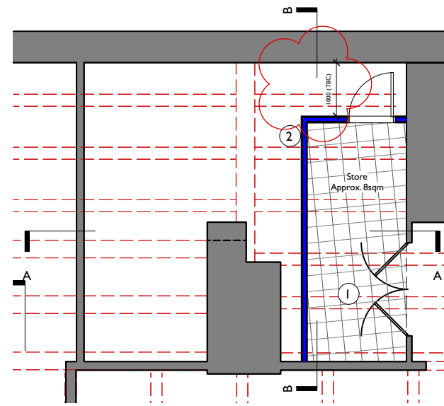
5 Proposed Plan - M&E Removed for Clarity Scale: 1:100
