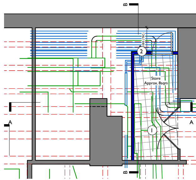
2 Pin 038:38 (partition), A1038:30 (door) Scale: 1:100
