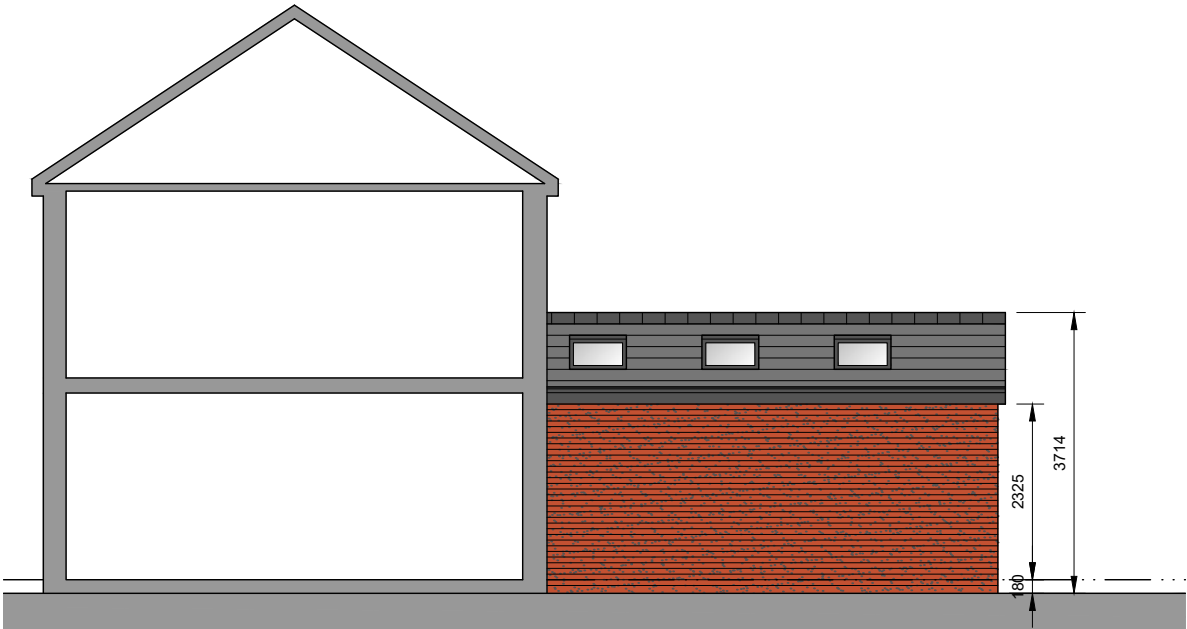
East Facing Side Elevational Section
