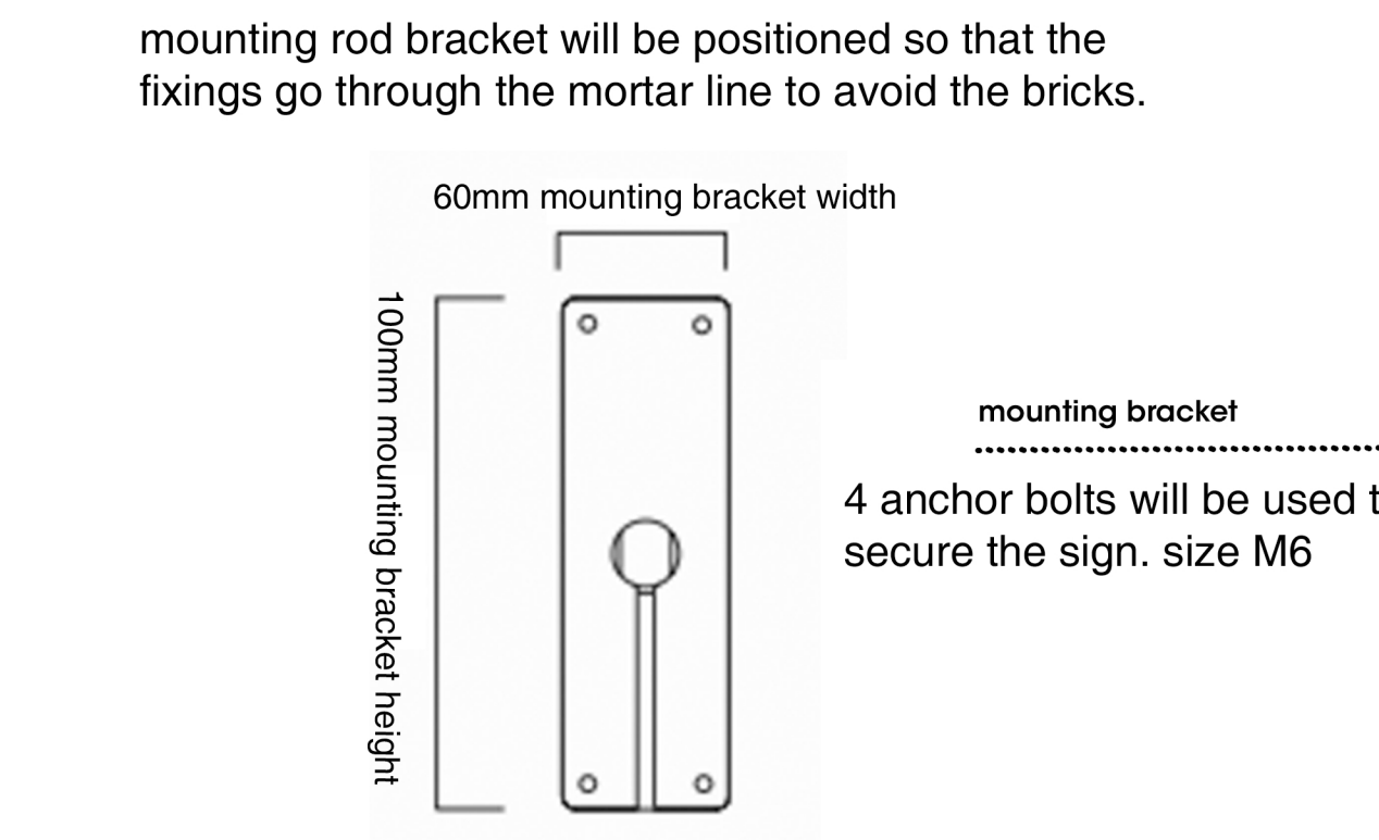
Anchor bolt sizes and cross section
