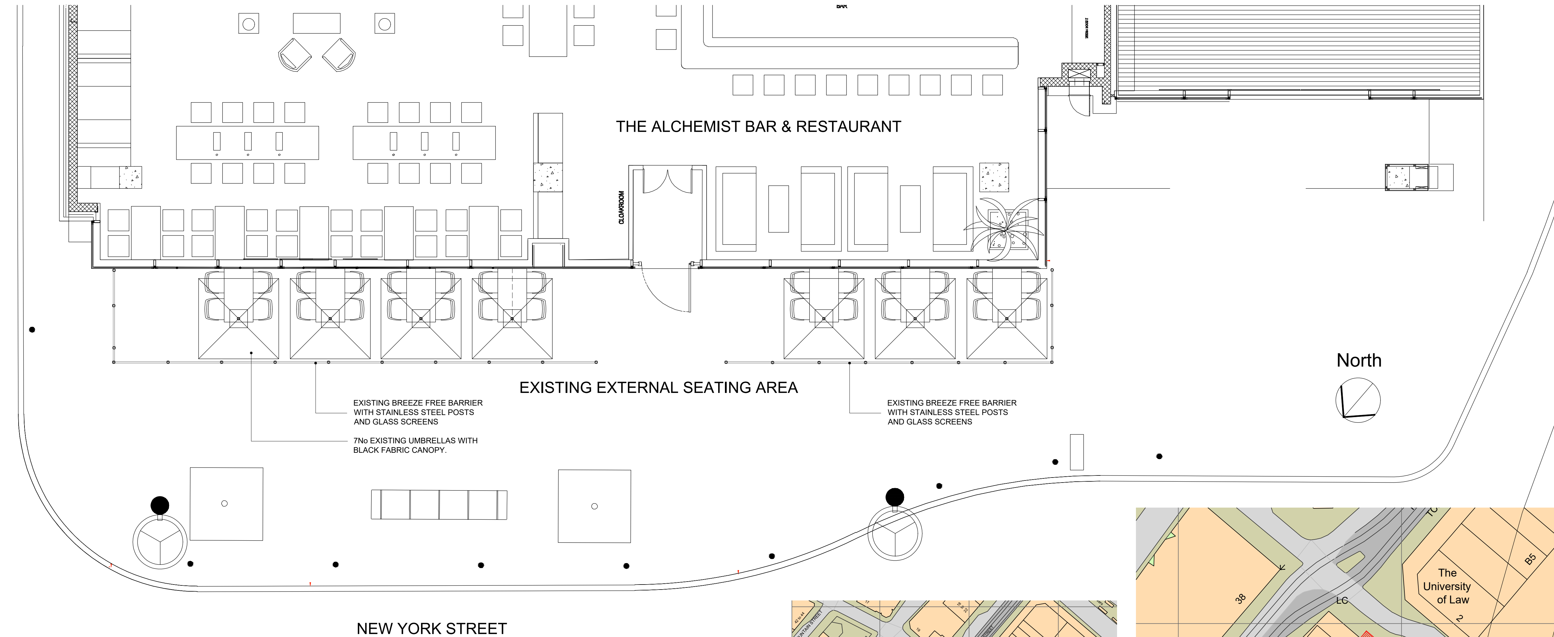
02 EXISTING PLAN
