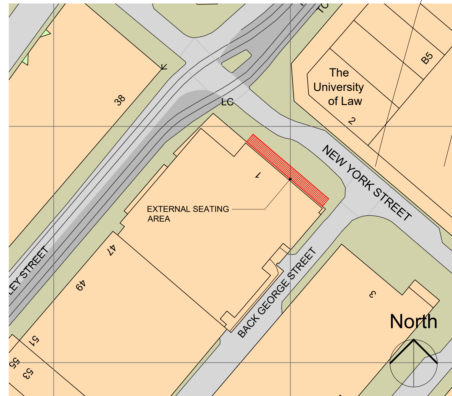
04 SITE BLOCK PLAN
