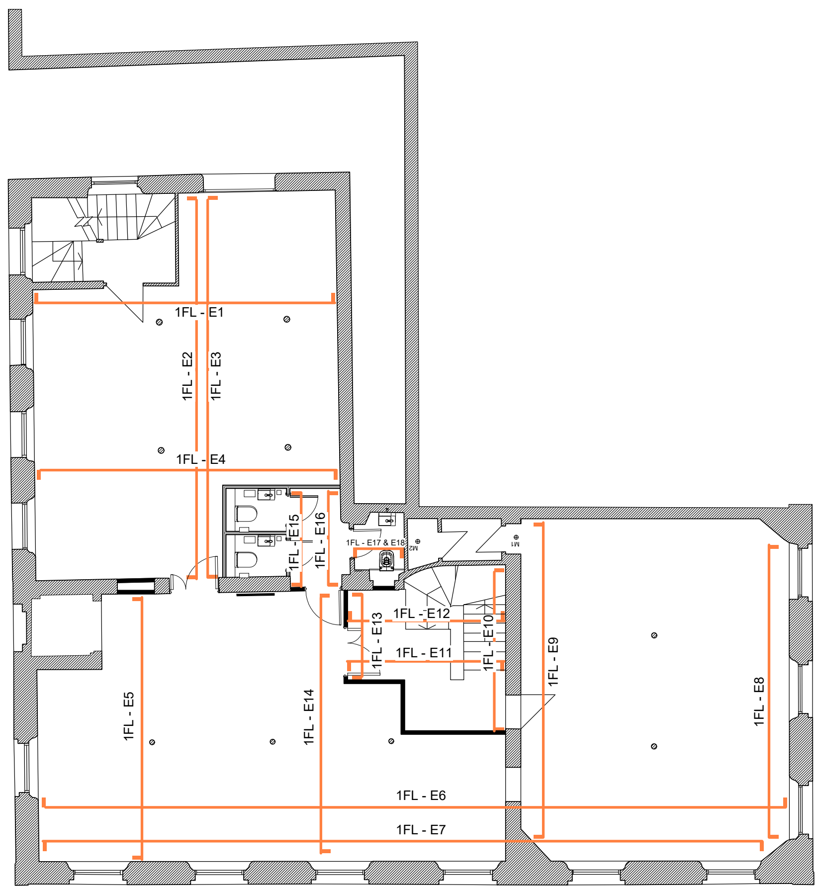
1FL Proposed Internal Elevation Layout_01 1 : 100
