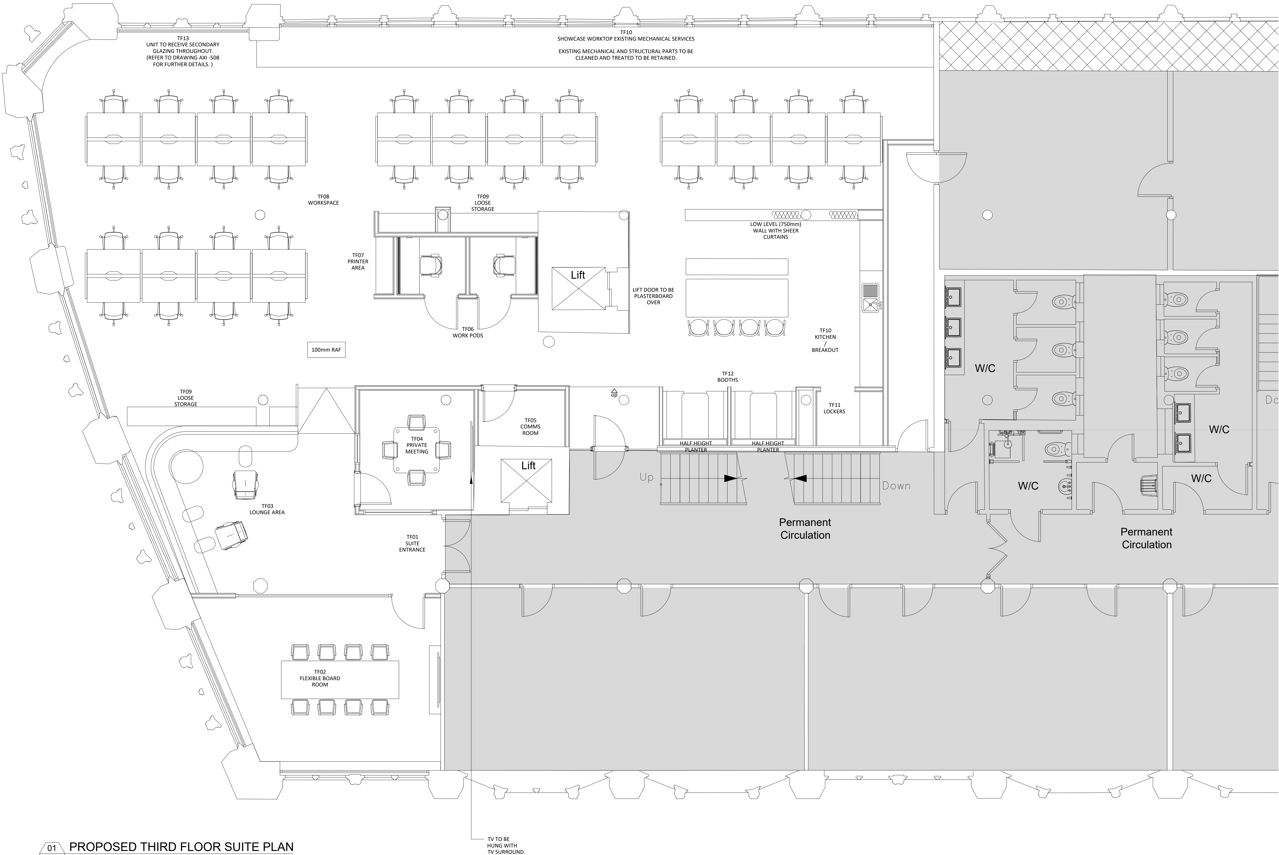
01 103 PROPOSED THIRD FLOOR SUITE PLAN SCALE - 1:50 @ A1
