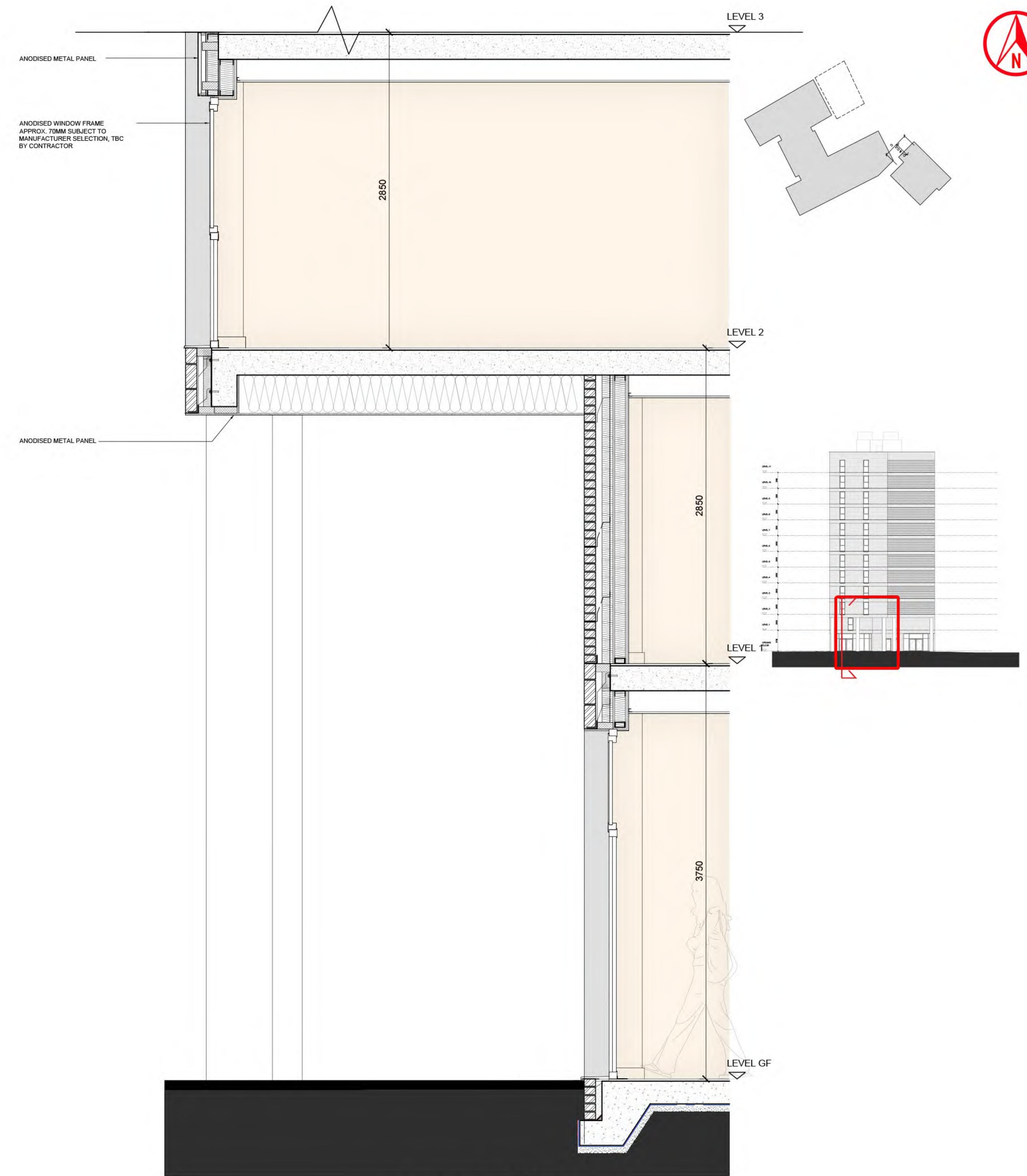
EXTERNAL WALL DETAIL SECTION C-2
