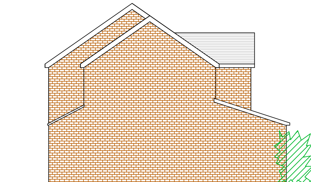
PROPOSED RHS ELEVATION
