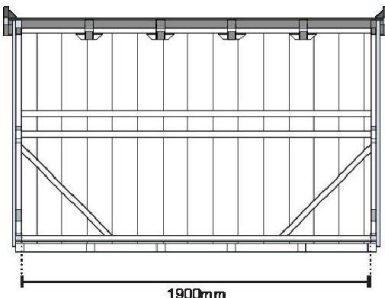
LONG SECTION
