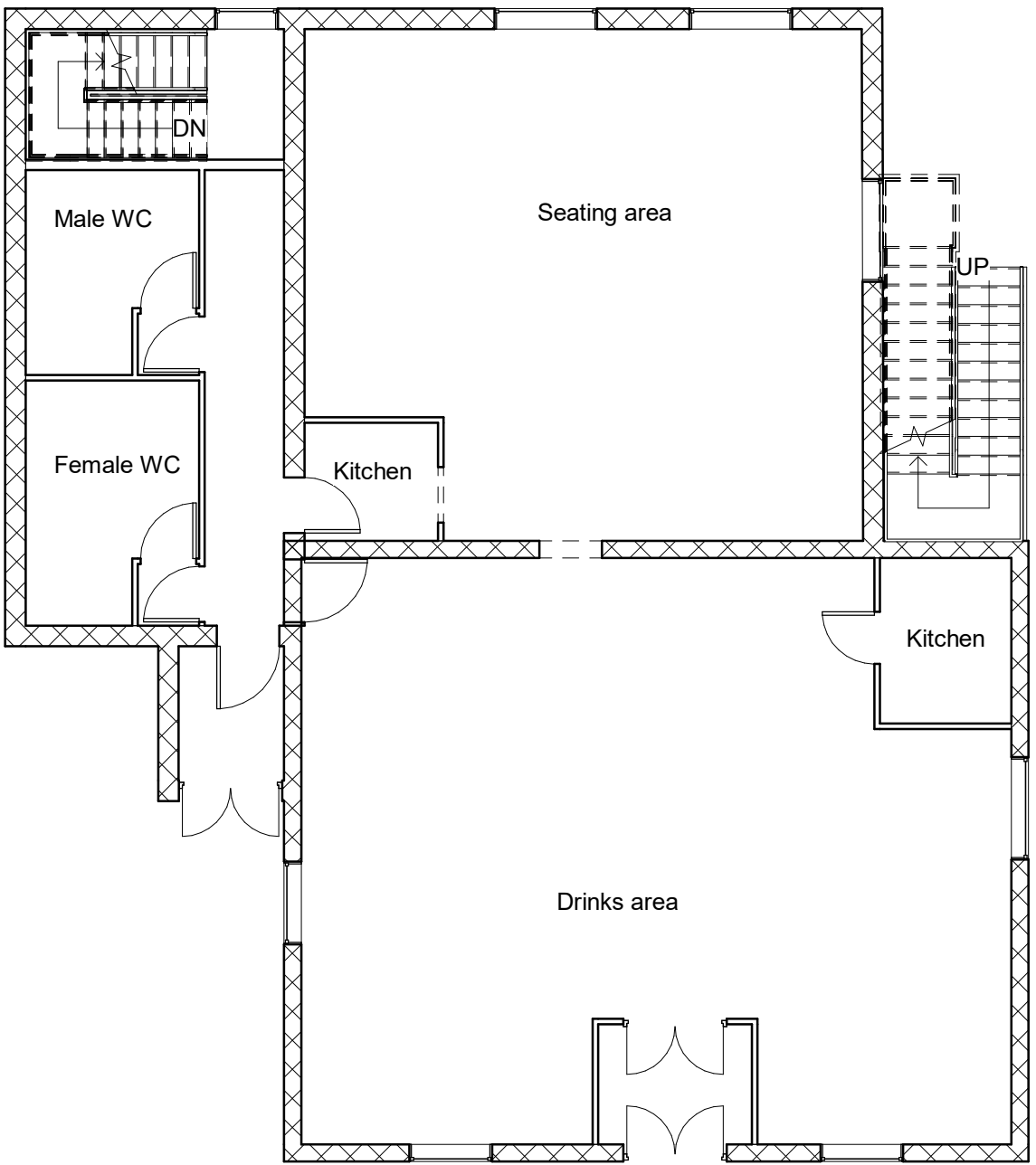
3 Ground Floor - Existing 1 : 100
