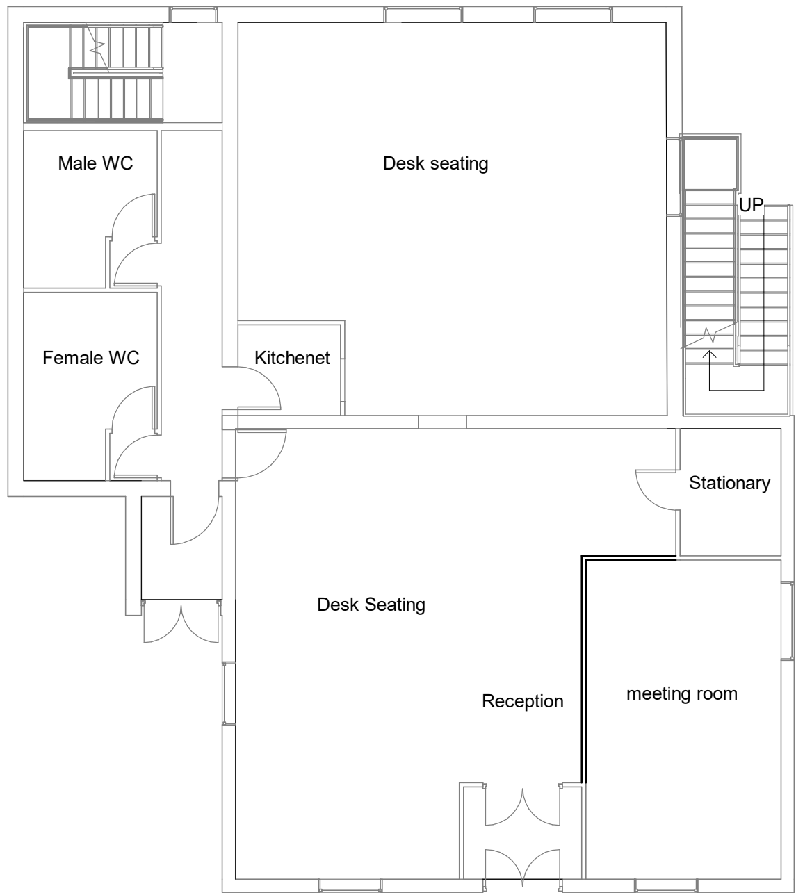
4 Ground Floor - Proposed 1 : 100
