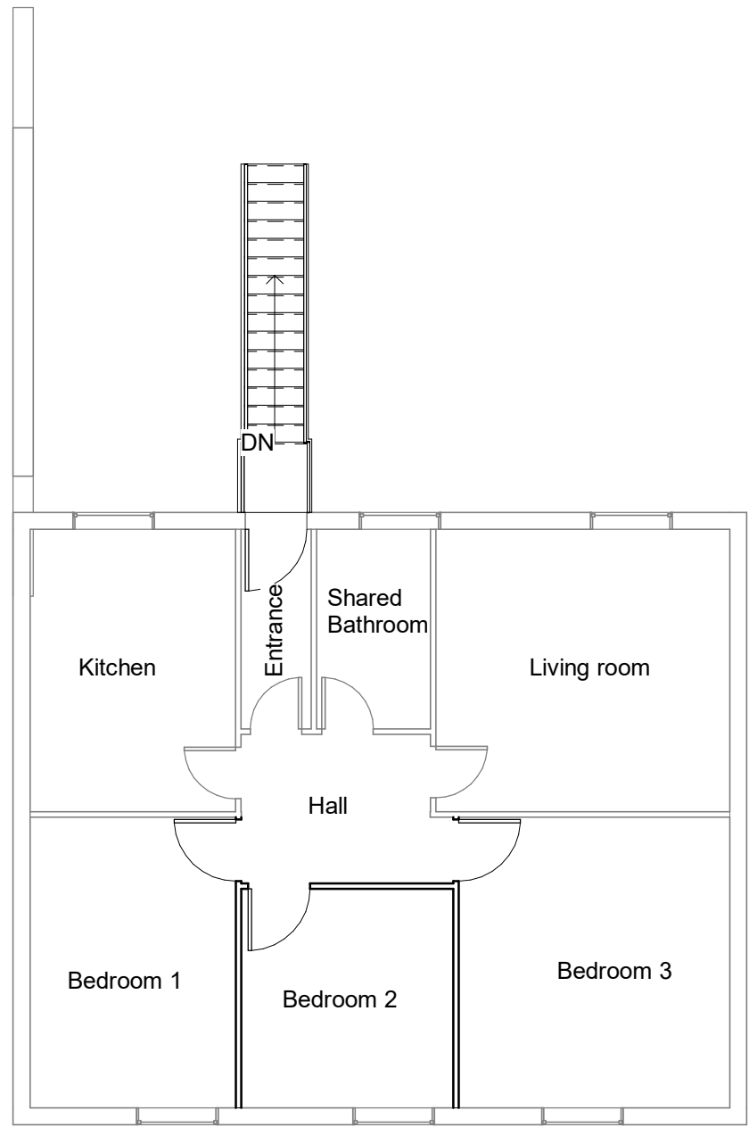
8 Second Floor - Proposed 1 : 100
