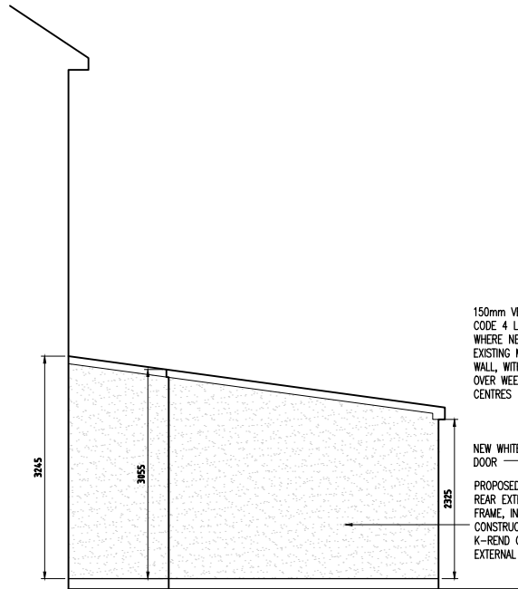
PROPOSED REAR/SIDE ELEVATION 1:100 @ A3
