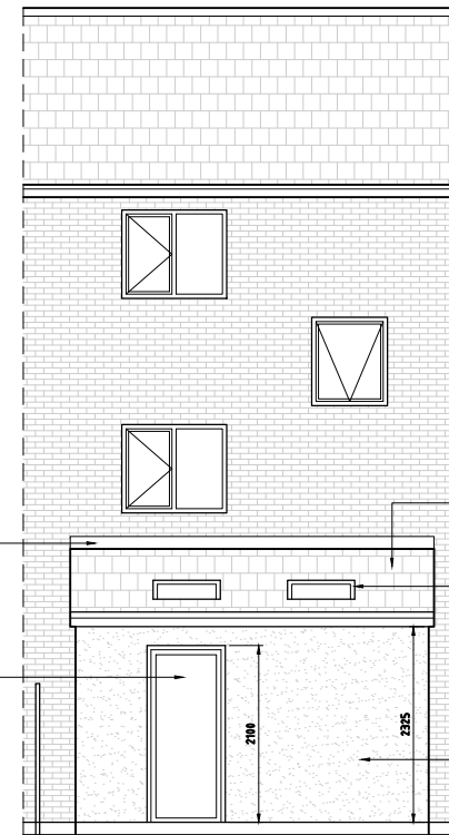
PROPOSED REAR ELEVATION 1:100 @ A3
