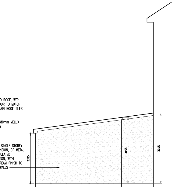
PROPOSED REAR/SIDE ELEVATION 1:100 @ A3
