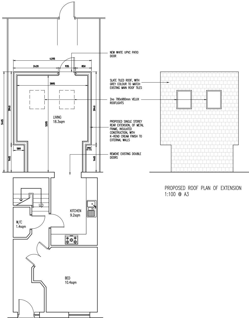
PROPOSED GROUND FLOOR PLAN 1:100 @ A3
