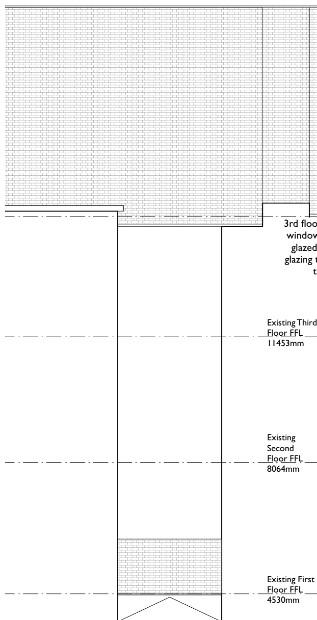
Lightwell Elevation BB Scale 1:100
