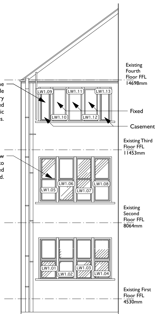
Lightwell Elevation CC Scale 1:100
