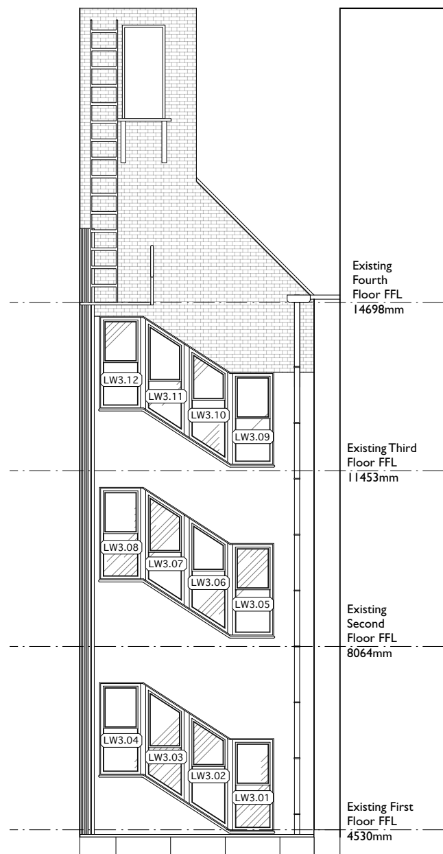
Lightwell Elevation AA Scale 1:100
