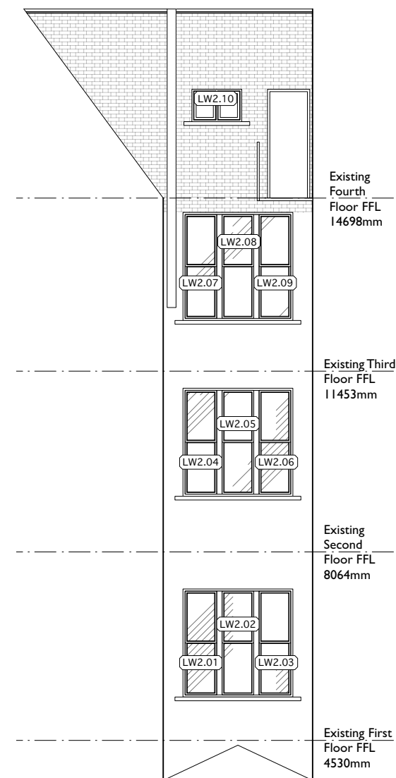
Lightwell Elevation DD Scale 1:100
