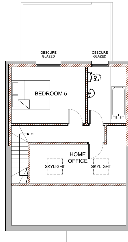
SECOND FLOOR PLAN 1:100
