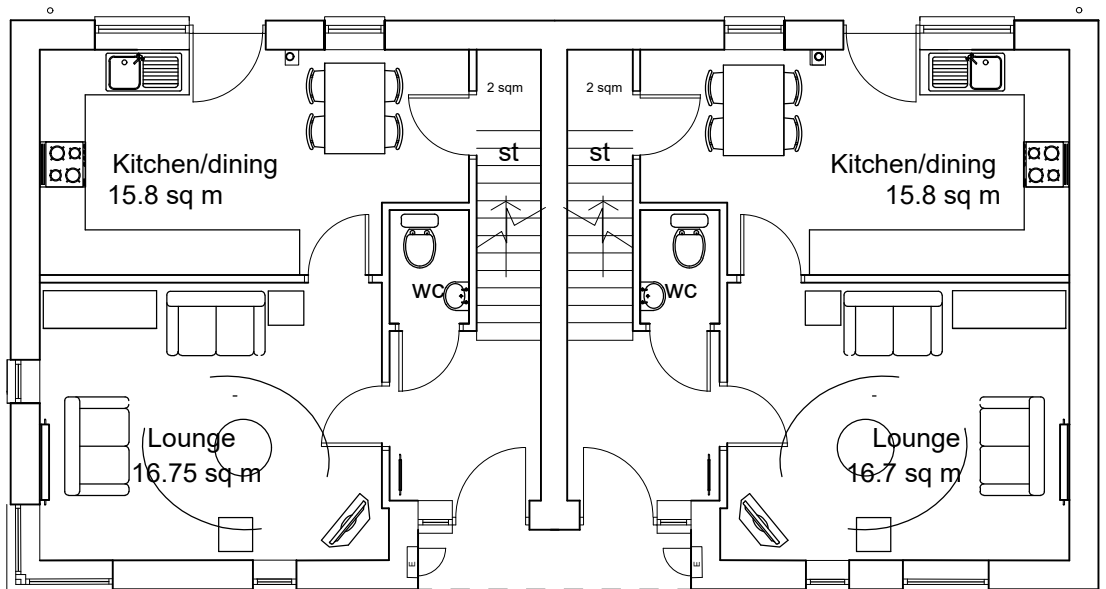
Ground floor 3b4p 88 sq m PLOT 16 E1
