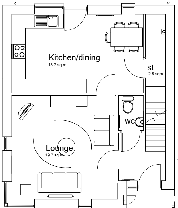
Ground floor 4b5p 101 sq m PLOT 15 D
