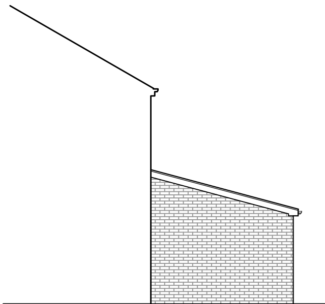
Proposed Side Elevation facing 2 Lynton Drive
