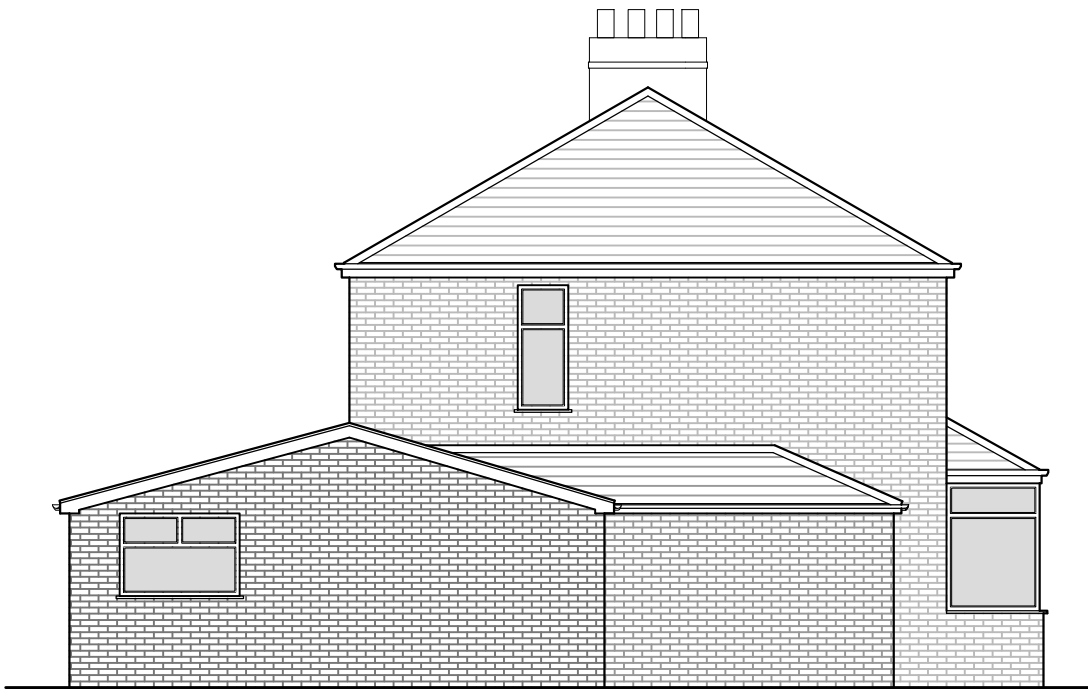
Porposed Side Elevation
