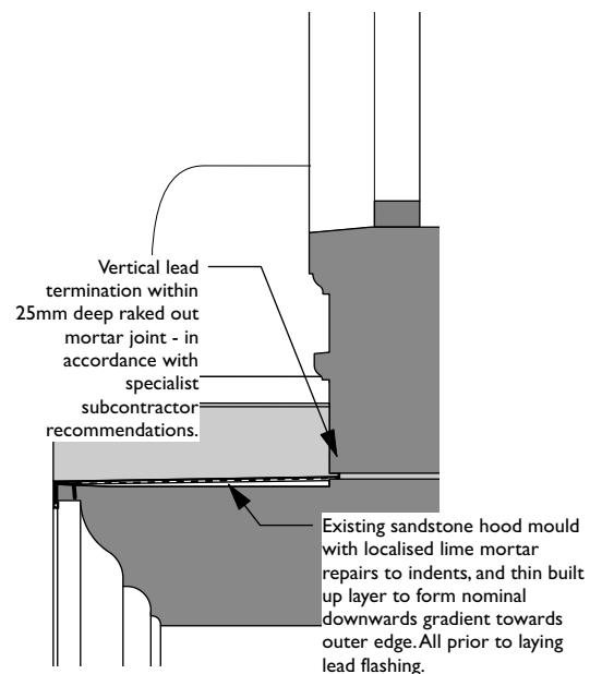
4 Proposed - Section BB Scale: 1:20
