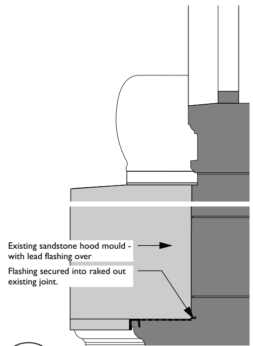
5 Proposed - Section CC Scale: 1:20
