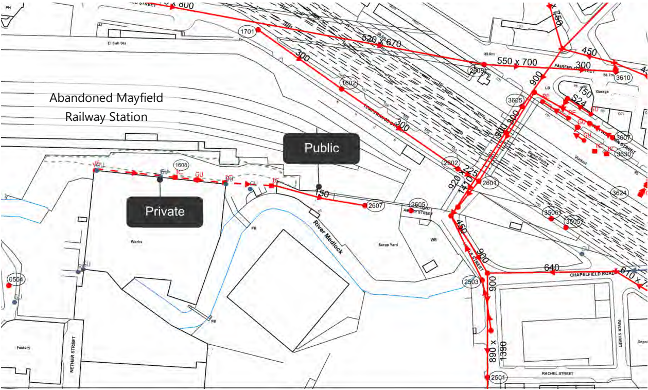
Figure 5-2 Location of the 150mm Combined Sewer on United Utilities Record Drawing (Image courtesy of the United Utilities © United Utilities Water PLC 2017)
