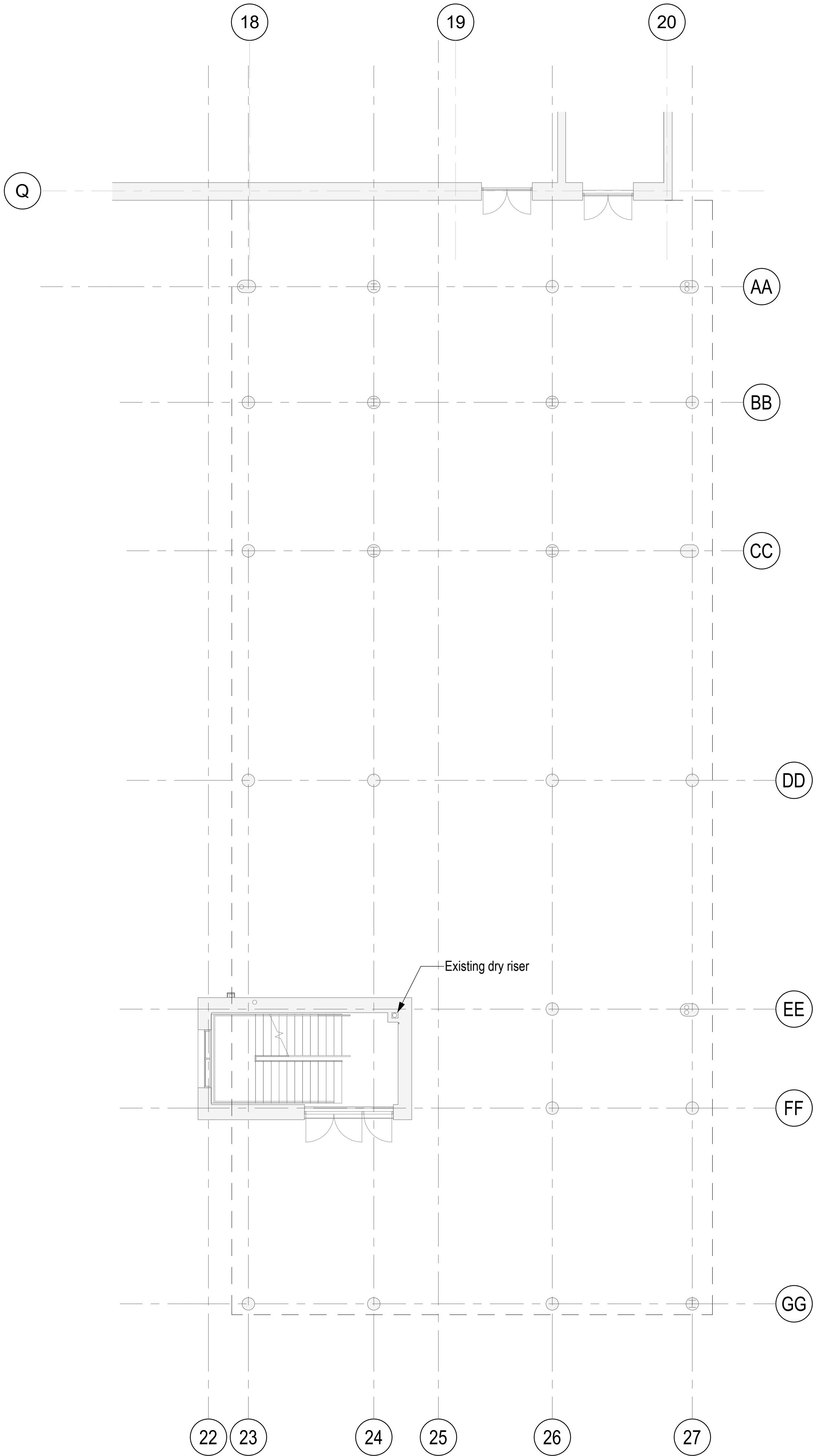
LEVEL 0 EXISTING PLAN
