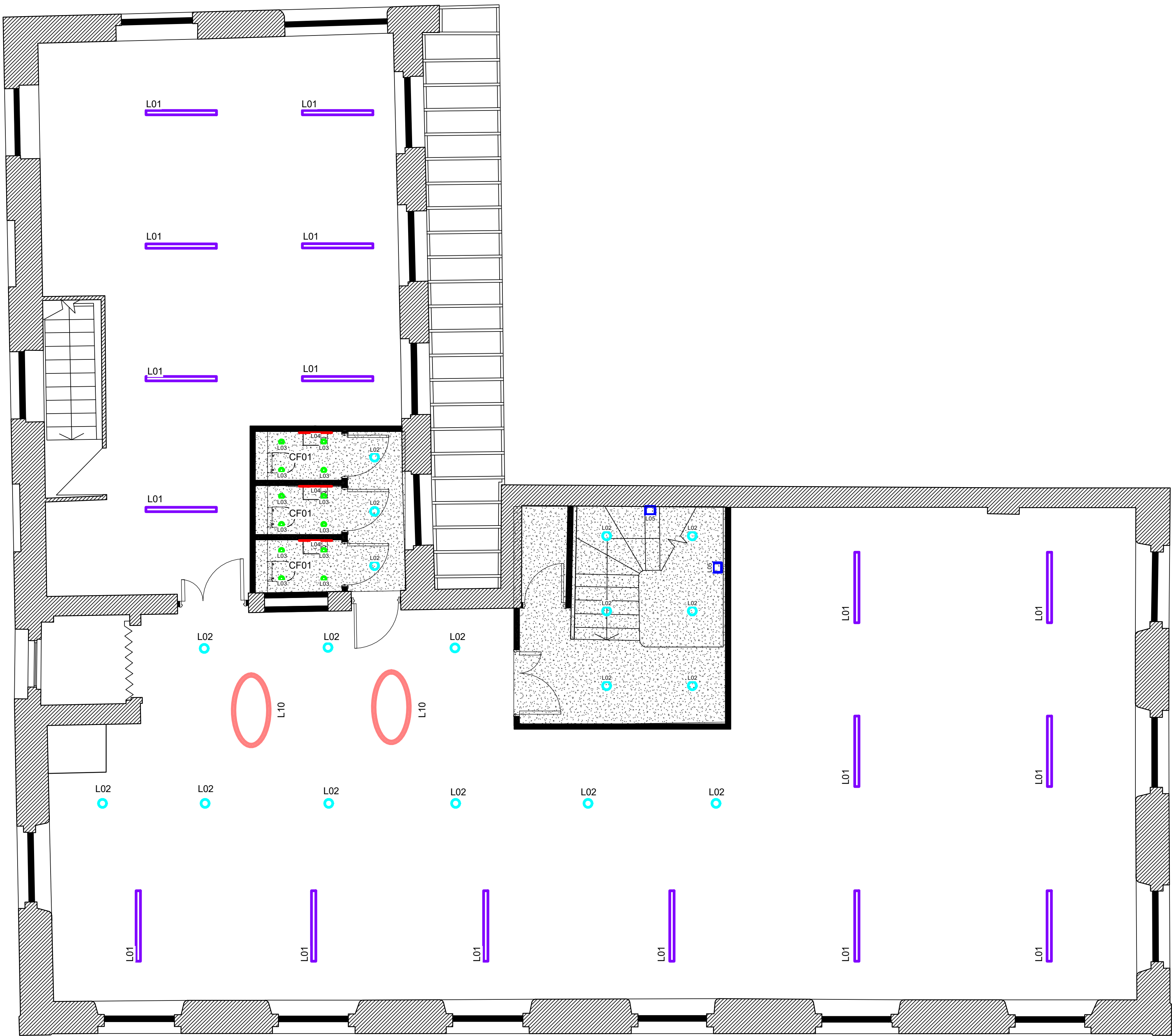
4FL Proposed Reflected Ceiling Layout Option 1 1 : 50
