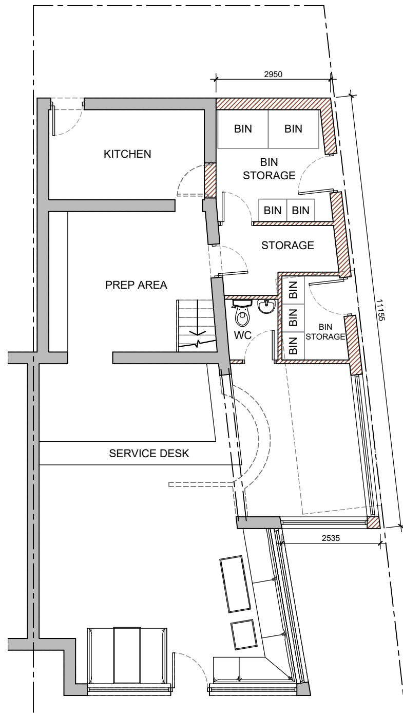
GROUND FLOOR 1:100
