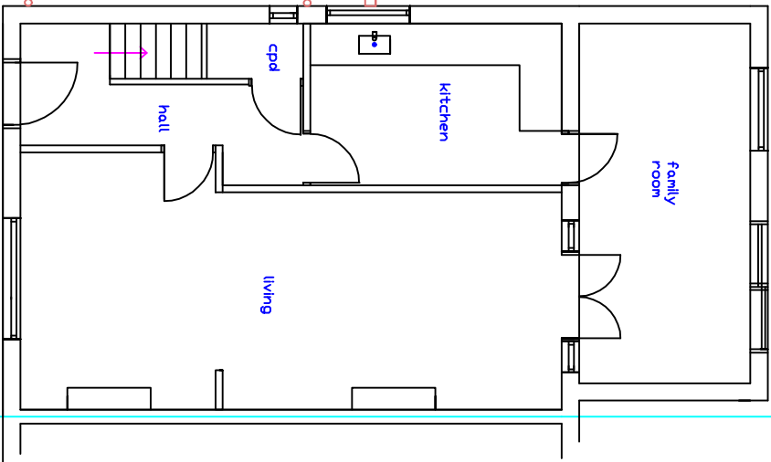
PROPOSED GROUND FLOOR 1:100
