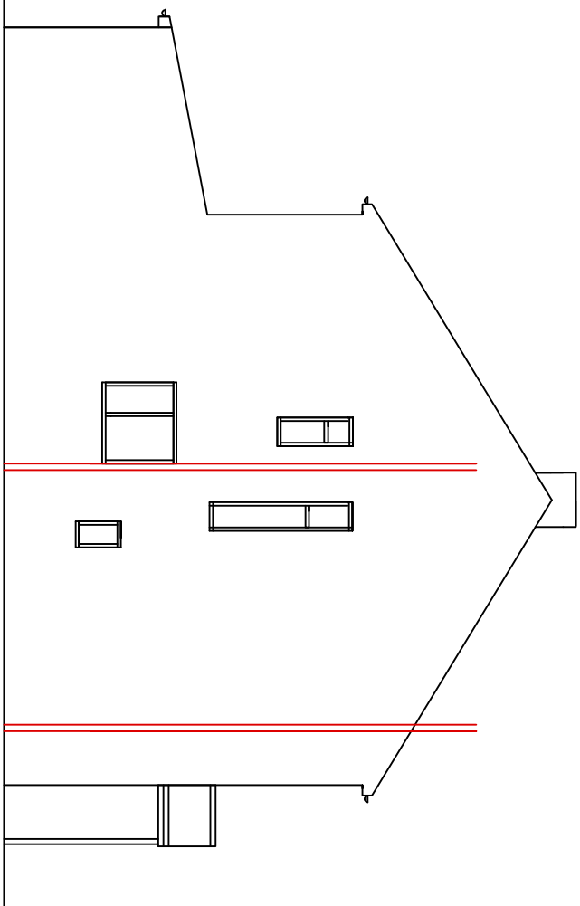
PROPOSED SIDE VIEW A 1:100
