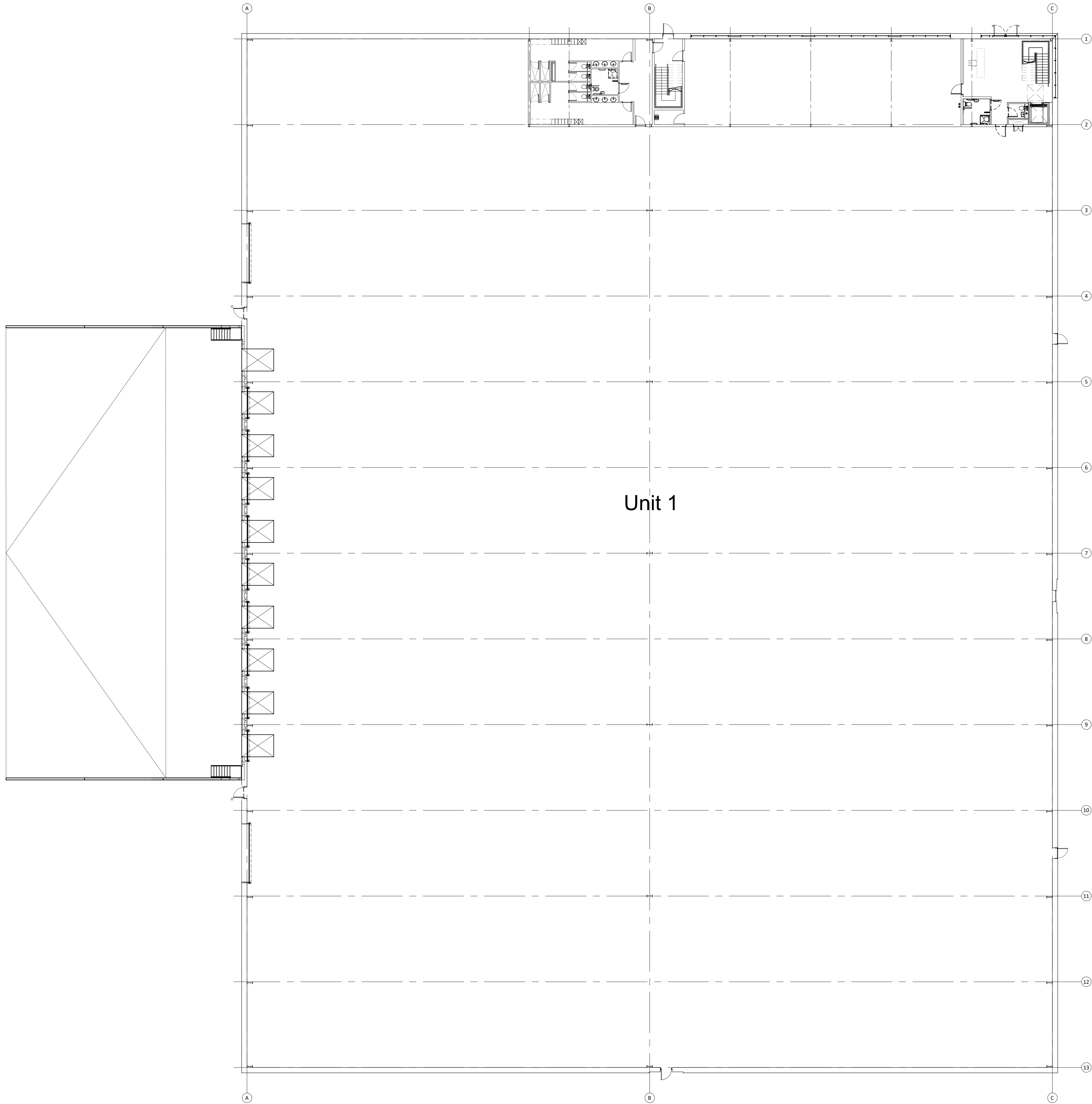
01 Unit 1 - Ground Floor GA Plan
