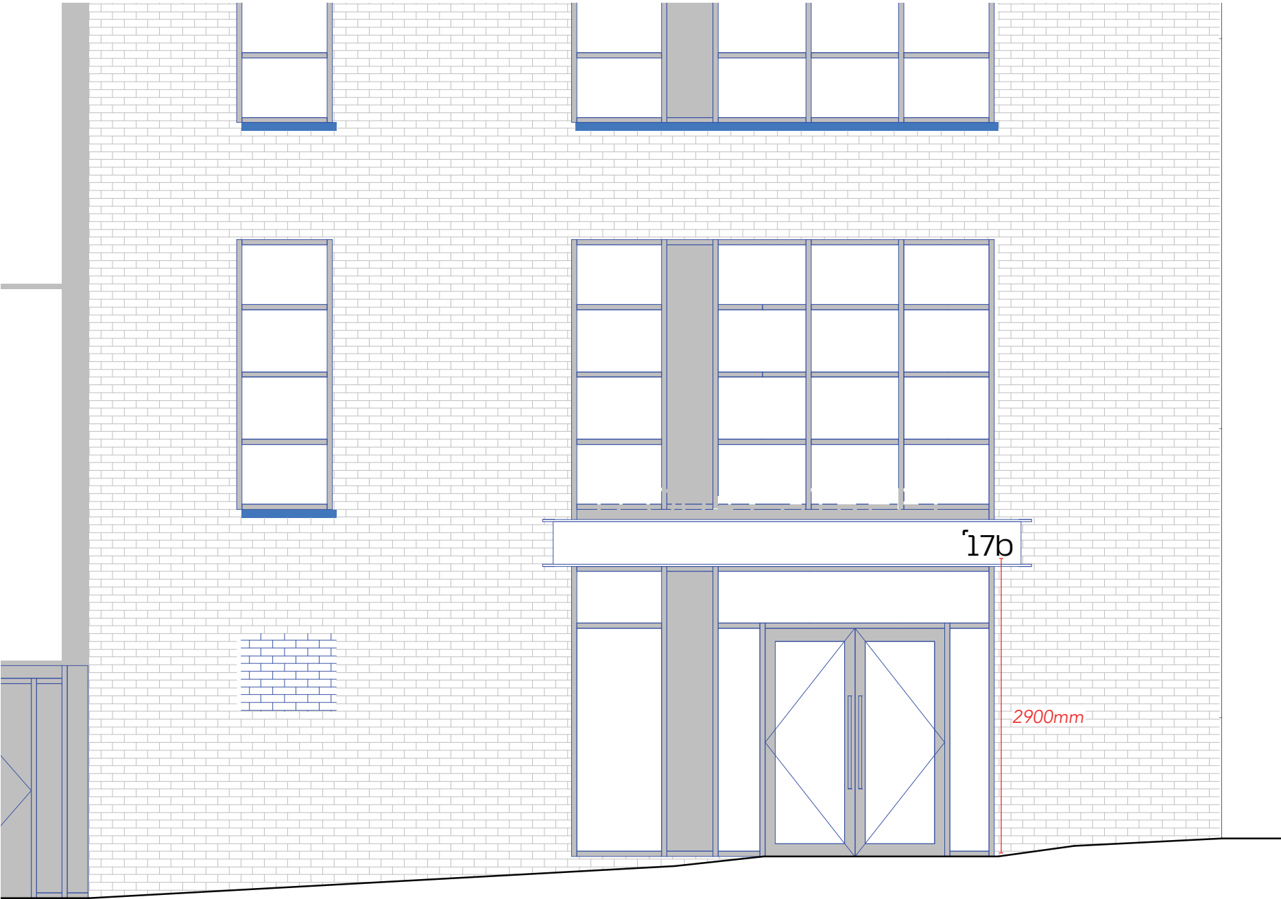
Indicative scale – 1:50
