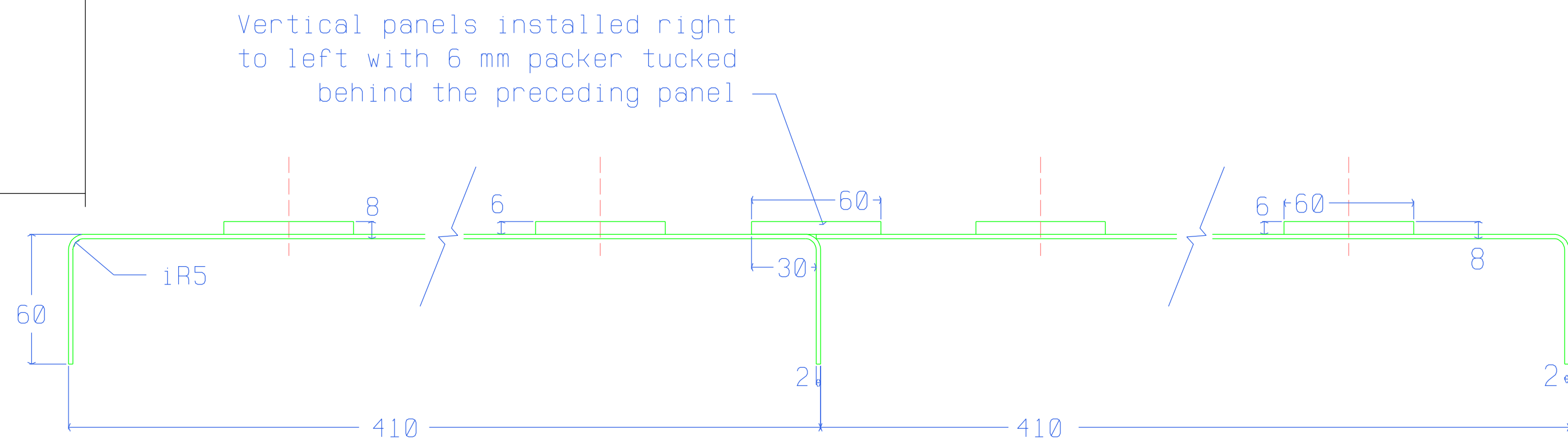
PANELS INTER-CONNECTION DETAIL - SCALE 1:2
