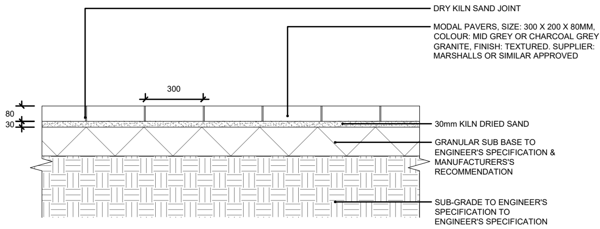
01A MODAL PAVING SETTS 600 SECTION
