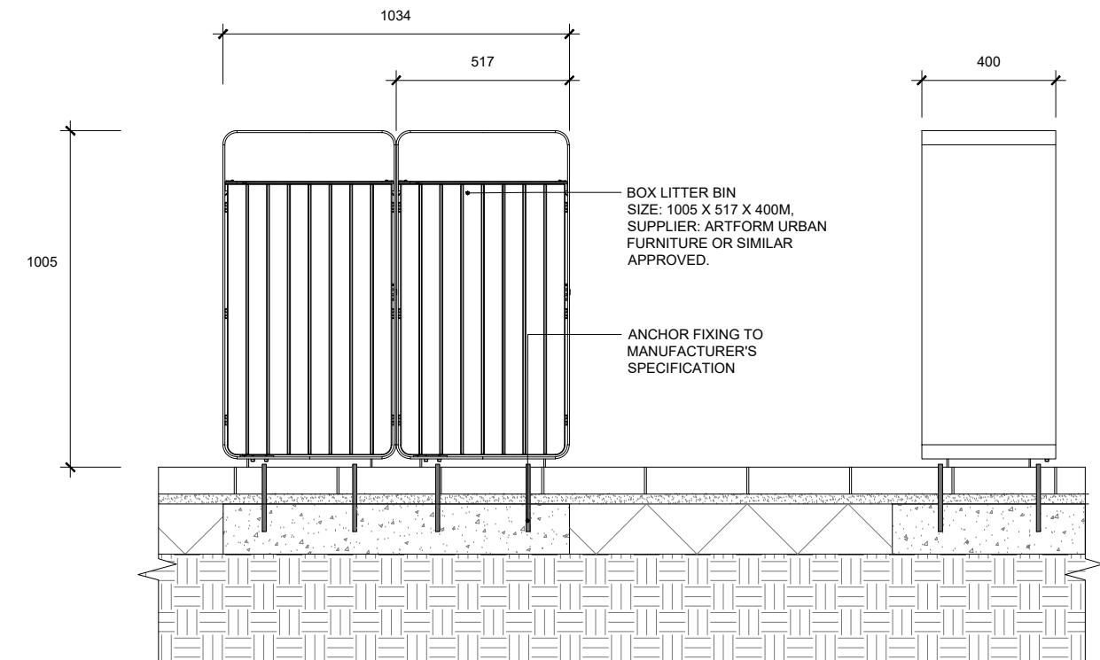
05A BOX LITTER AND RECYCLE BIN 600 SECTION
