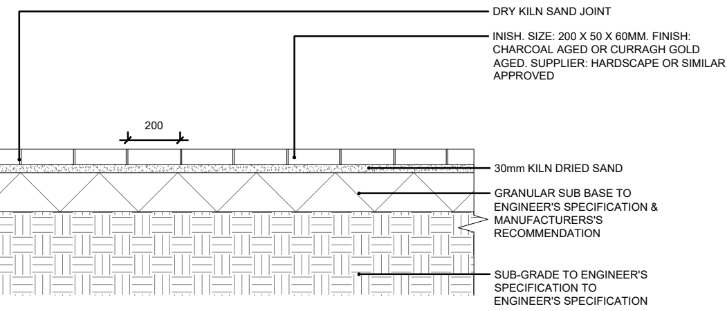
02A INISH CONCRETE PAVING 600 SECTION
