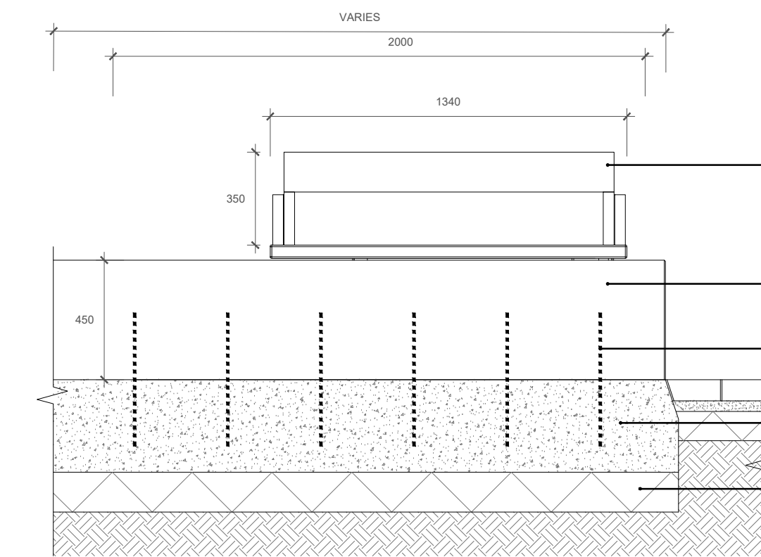
03A TIMBER TOP BENCH 600 SECTION
