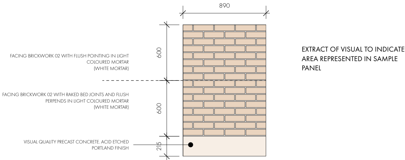
INITIAL SAMPLE PANEL TO BE CONSTRUCTED TO ESTABLISH MORTAR COLOUR AND POINTING 1:25
