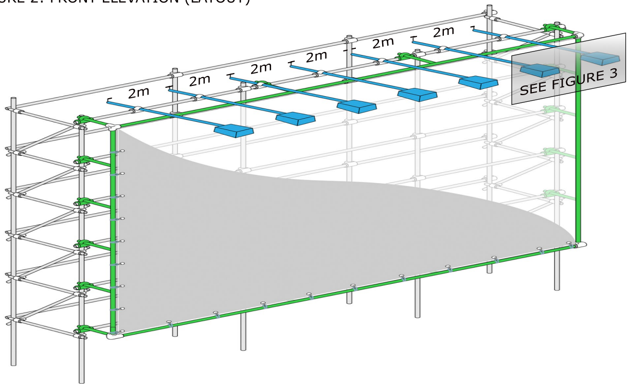
FIGURE 2: FRONT ELEVATION (LAYOUT)
