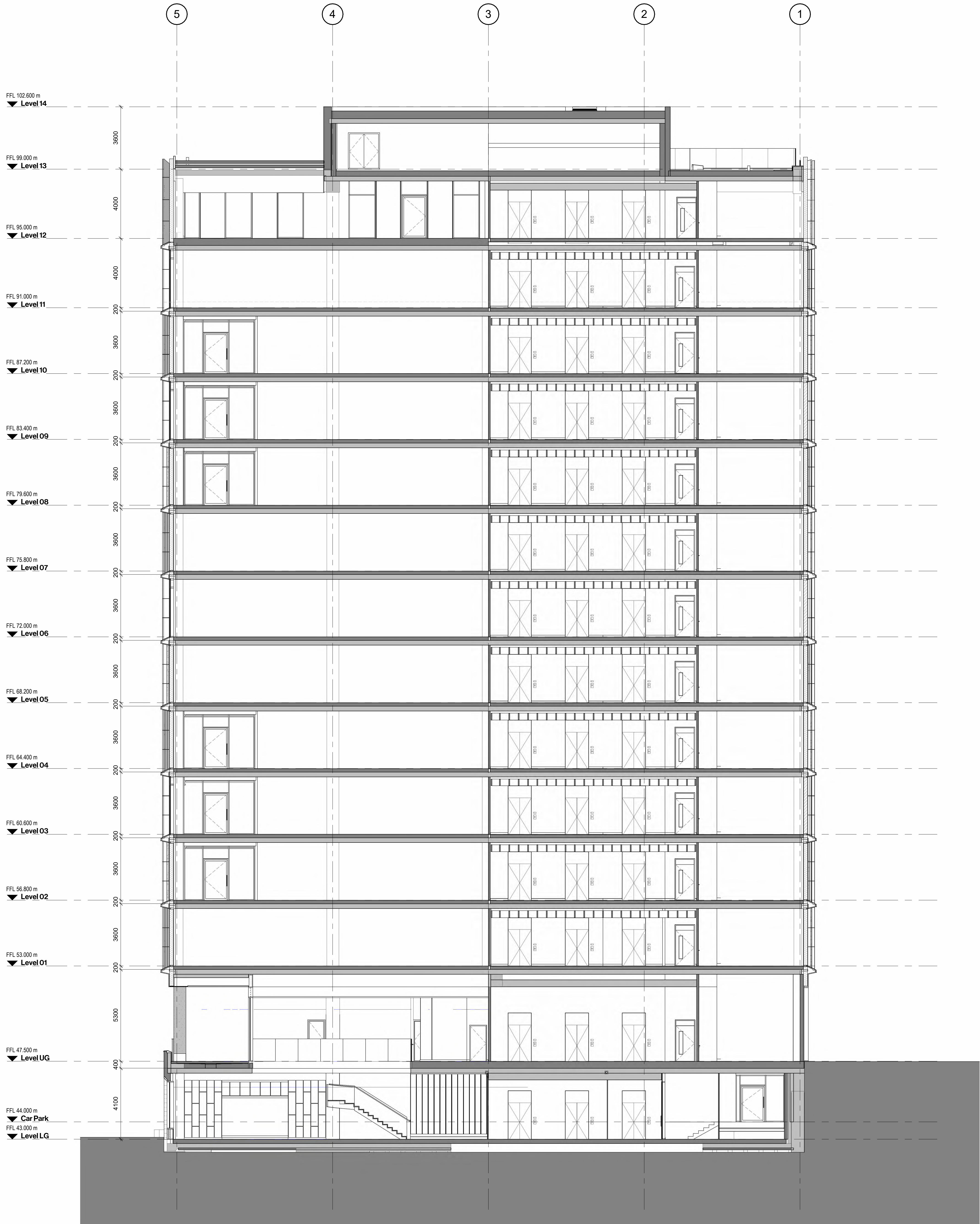
1 Section - BB
