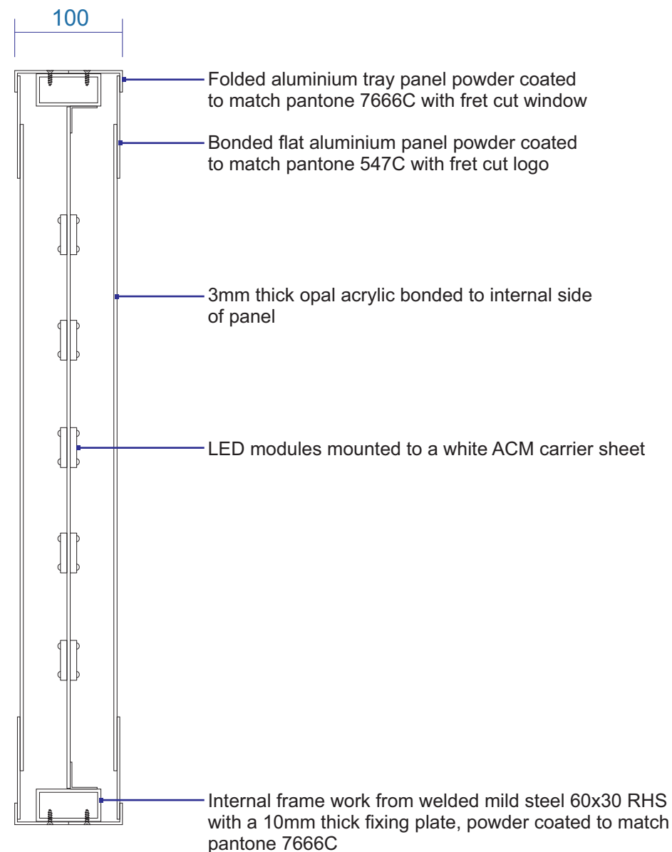
SECTION THROUGH SIGN B scale 1:5
