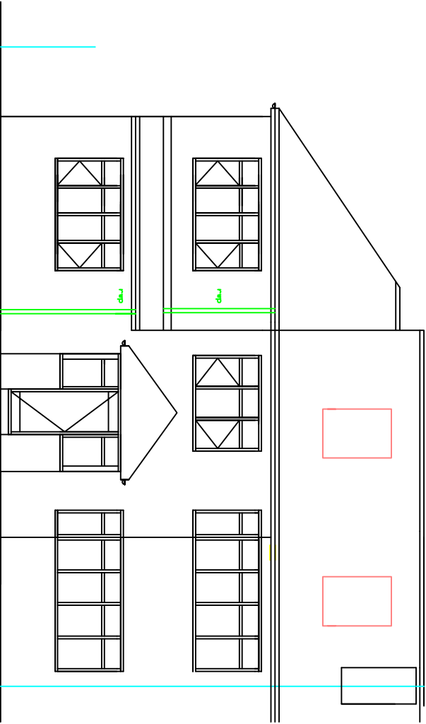
PROPOSED FRONT VIEW 1: 100
