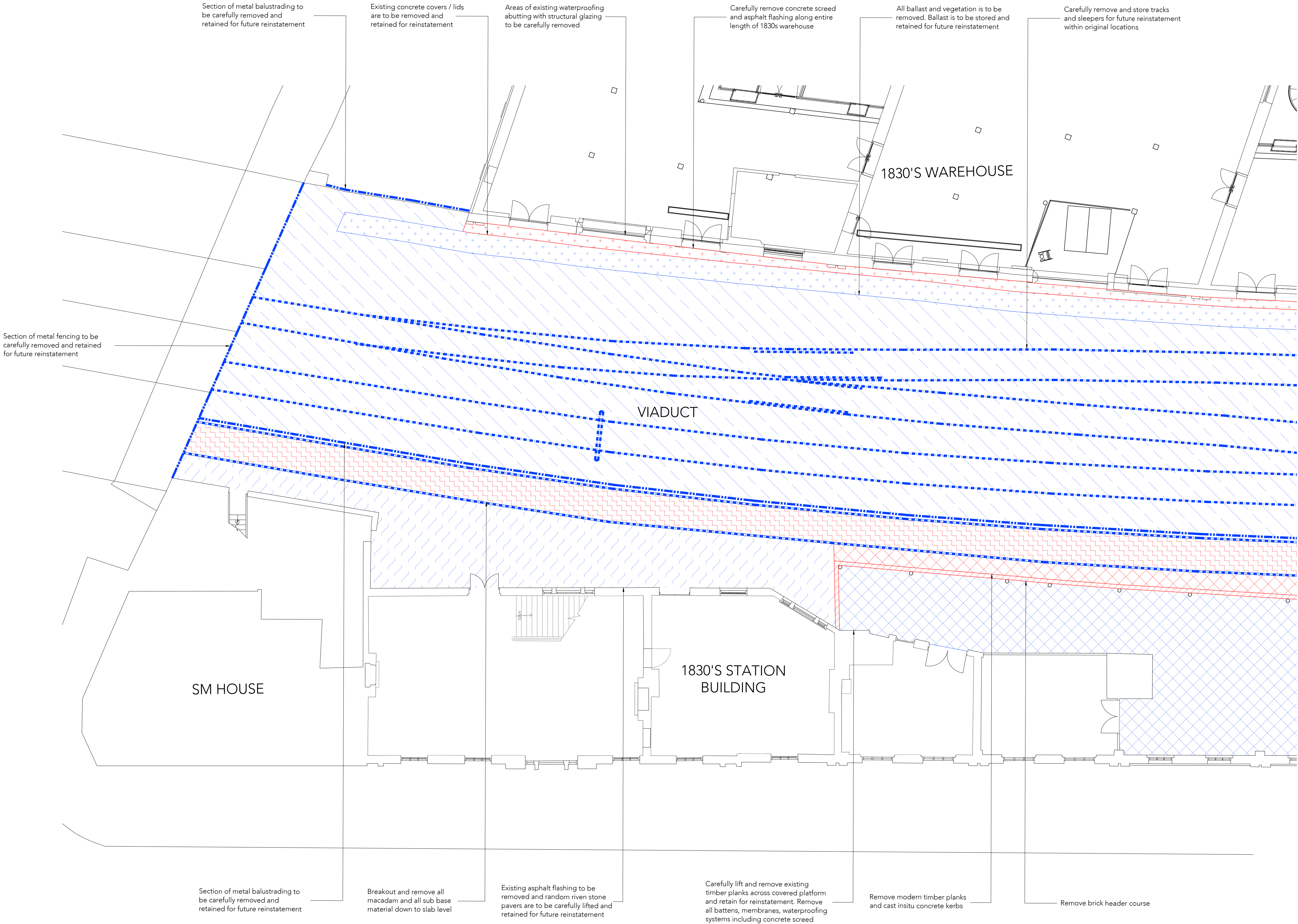
Site Plan - Demolition & Removals Plan 1 Scale 1:100
