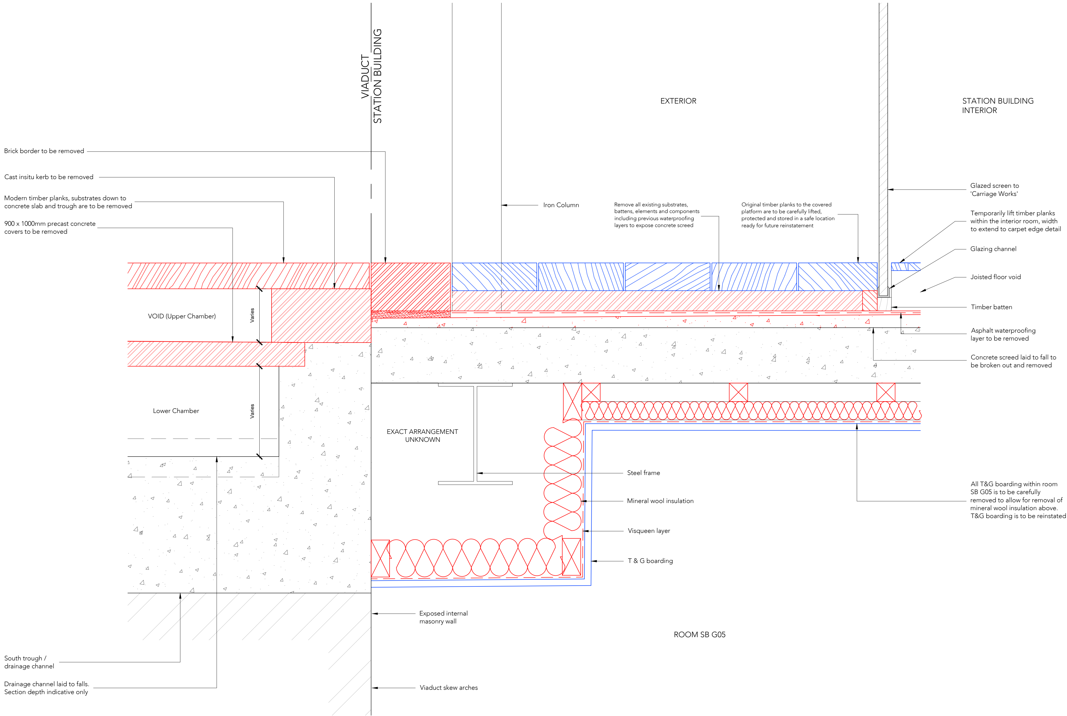
Typical Detail Through Glass Screen F-F Demolition & Removals Scale 1:5
