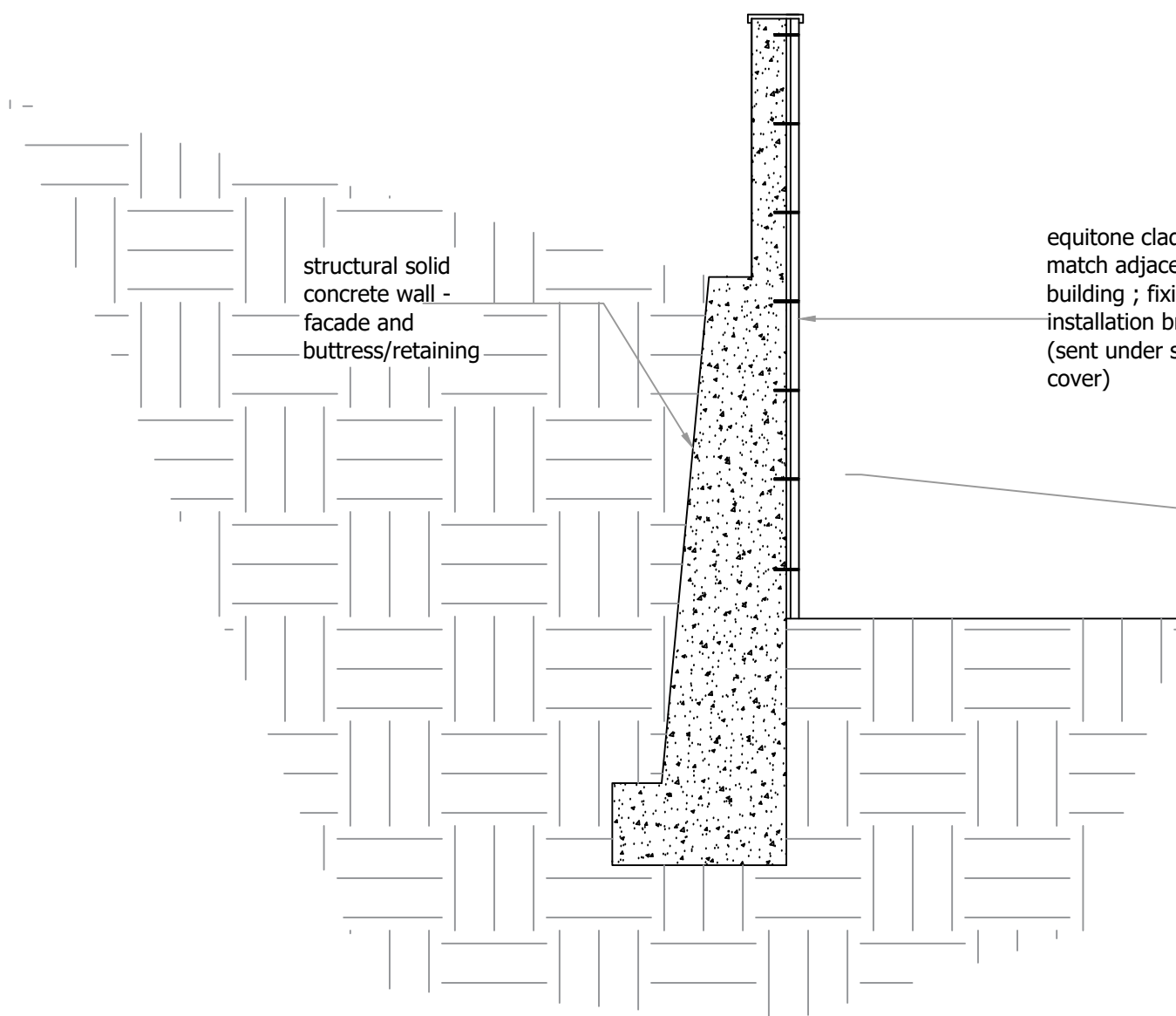
SECTION
