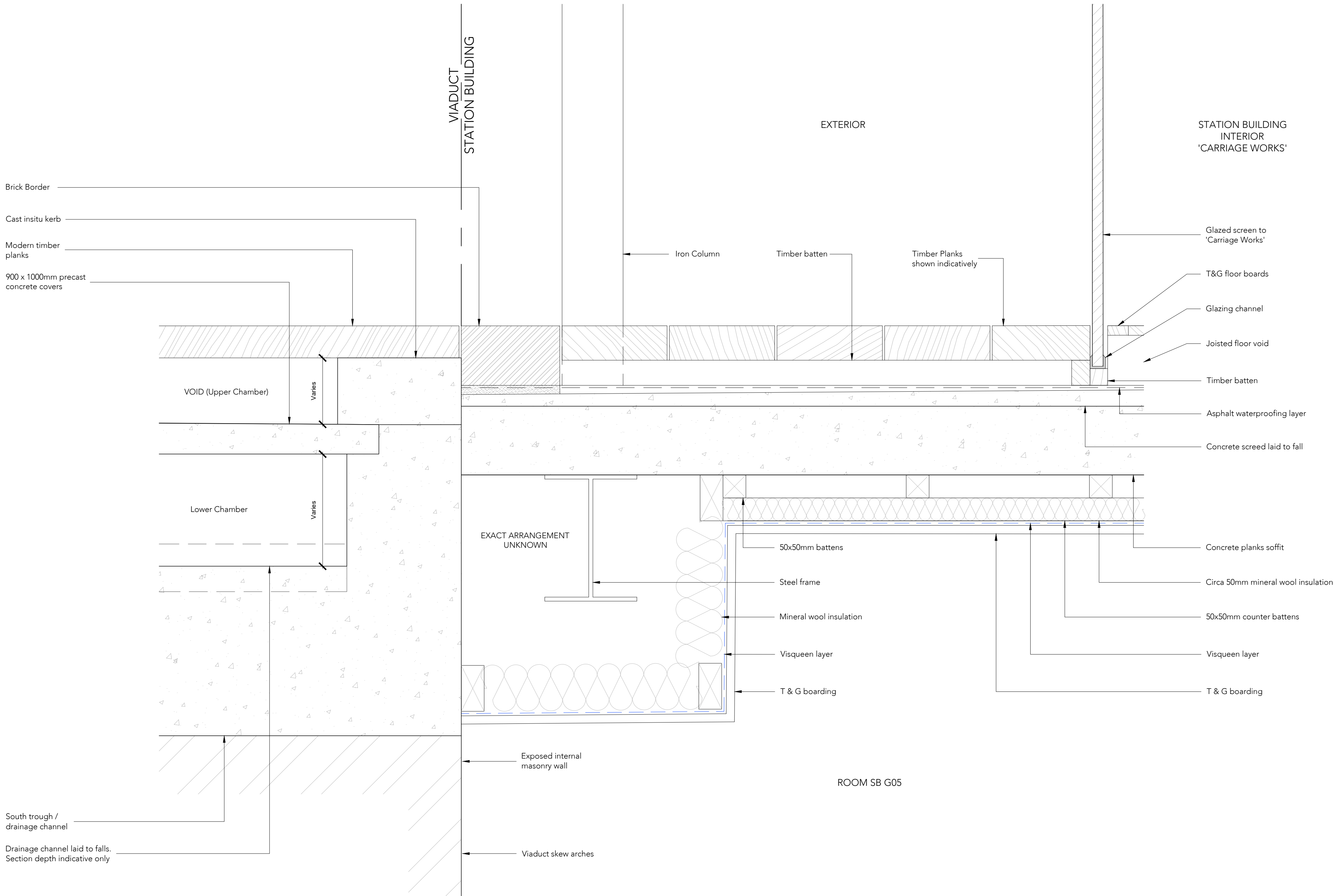
Typical detail through glass screen F-F as Existing Scale 1:5
