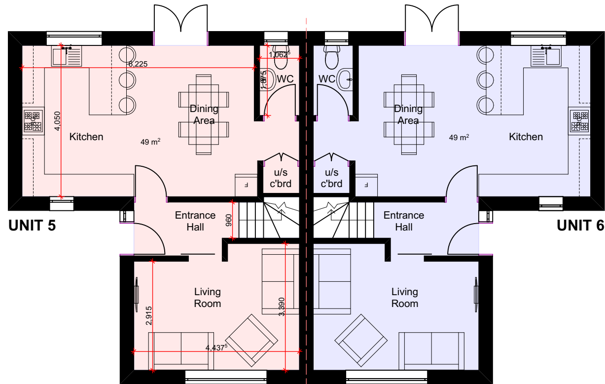
PROPOSED GA GROUND FLOOR PLAN
