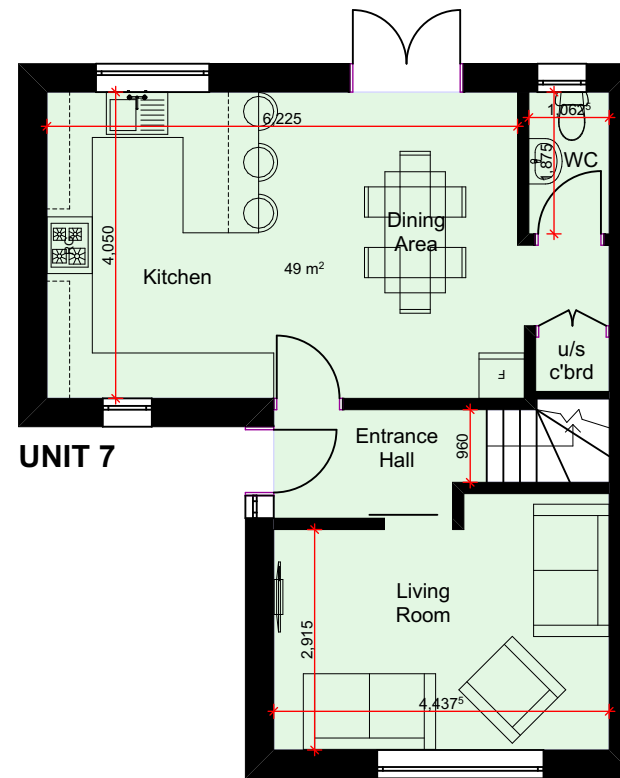
PROPOSED GA GROUND FLOOR PLAN
