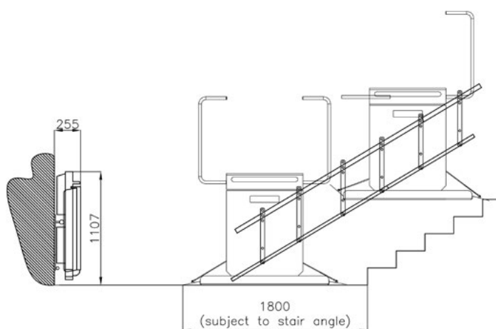
Options: upper rail extension (left) and fold down seat (right)
