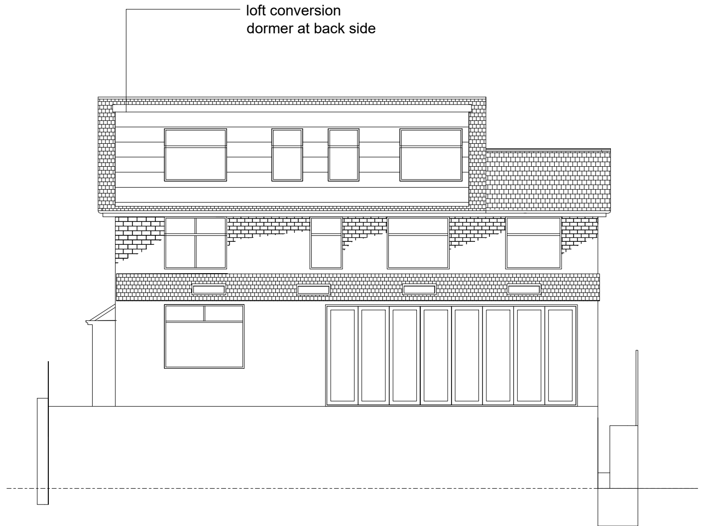
- ELEVATION - Back PROPOSED 1 : 100 ( IN A3)
